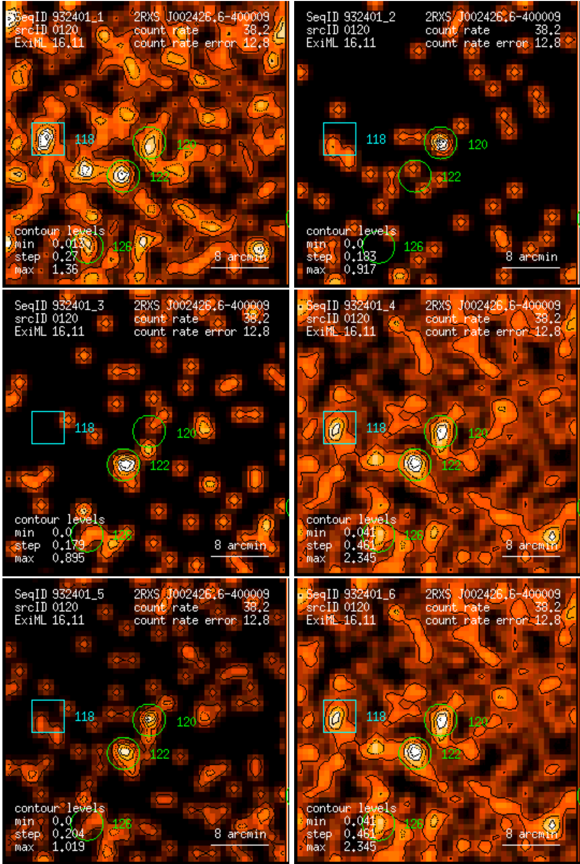
Figure 120: RASS 932401: detection 0120: band rate images, Gaussian filter: (1) PSPC channels 11 – 41, (2) 52 – 90, (3) 91 – 201, (4) 11 – 235, (5) 52 – 201, (6) 11 – 201. Broad band rates in counts/ks. Band rate contour levels in counts/ks/arcmin 2 .
