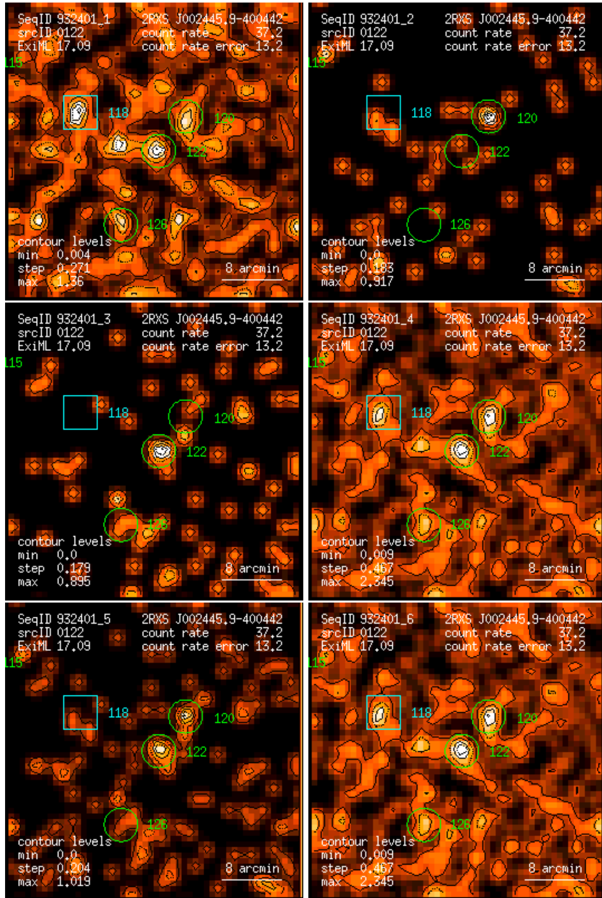
Figure 122: RASS 932401: detection 0122: band rate images, Gaussian filter: (1) PSPC channels 11 – 41, (2) 52 – 90, (3) 91 – 201, (4) 11 – 235, (5) 52 – 201, (6) 11 – 201. Broad band rates in counts/ks. Band rate contour levels in counts/ks/arcmin 2 .
