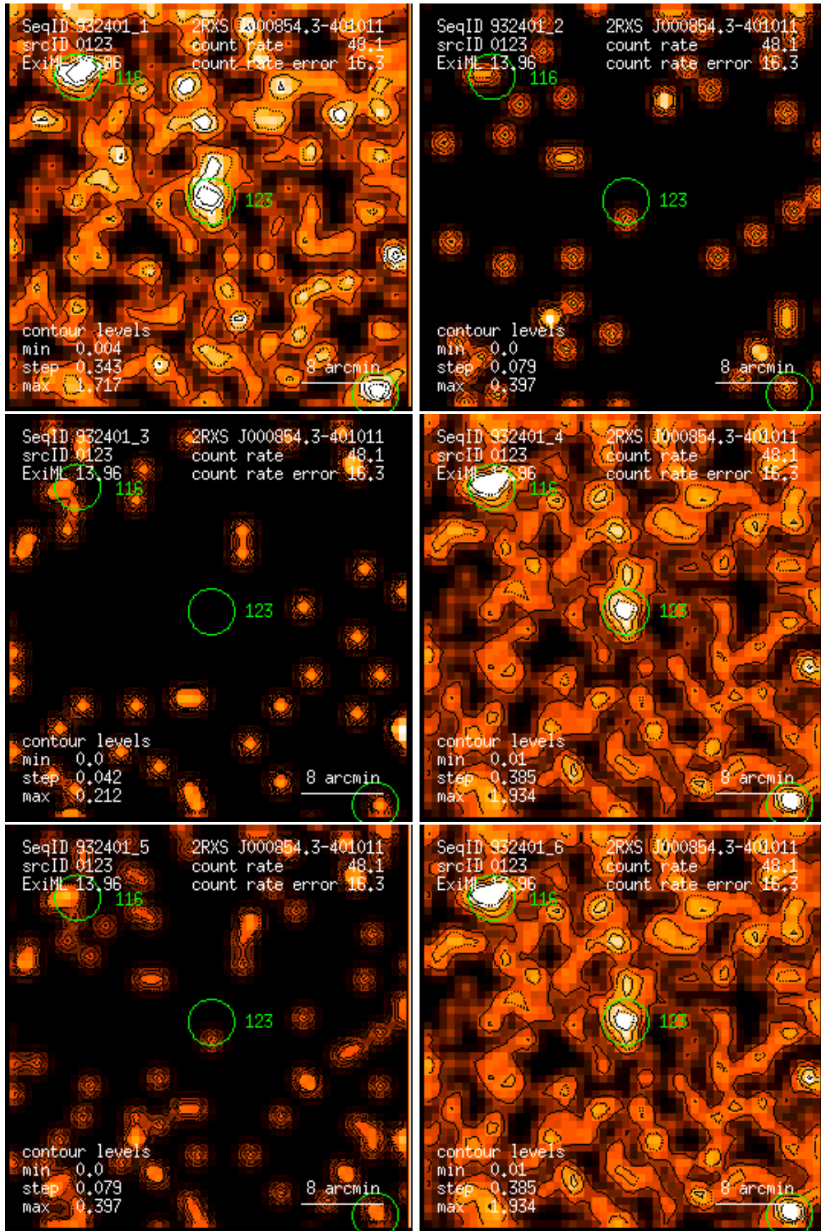
Figure 123: RASS 932401: detection 0123: band rate images, Gaussian filter: (1) PSPC channels 11 – 41, (2) 52 – 90, (3) 91 – 201, (4) 11 – 235, (5) 52 – 201, (6) 11 – 201. Broad band rates in counts/ks. Band rate contour levels in counts/ks/arcmin 2 .
