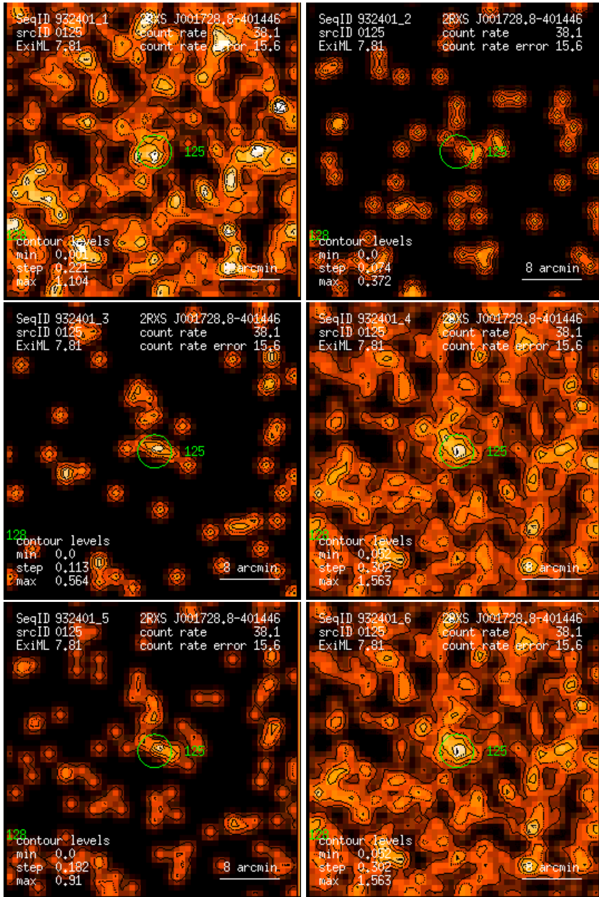
Figure 125: RASS 932401: detection 0125: band rate images, Gaussian filter: (1) PSPC channels 11 – 41, (2) 52 – 90, (3) 91 – 201, (4) 11 – 235, (5) 52 – 201, (6) 11 – 201. Broad band rates in counts/ks. Band rate contour levels in counts/ks/arcmin 2 .
