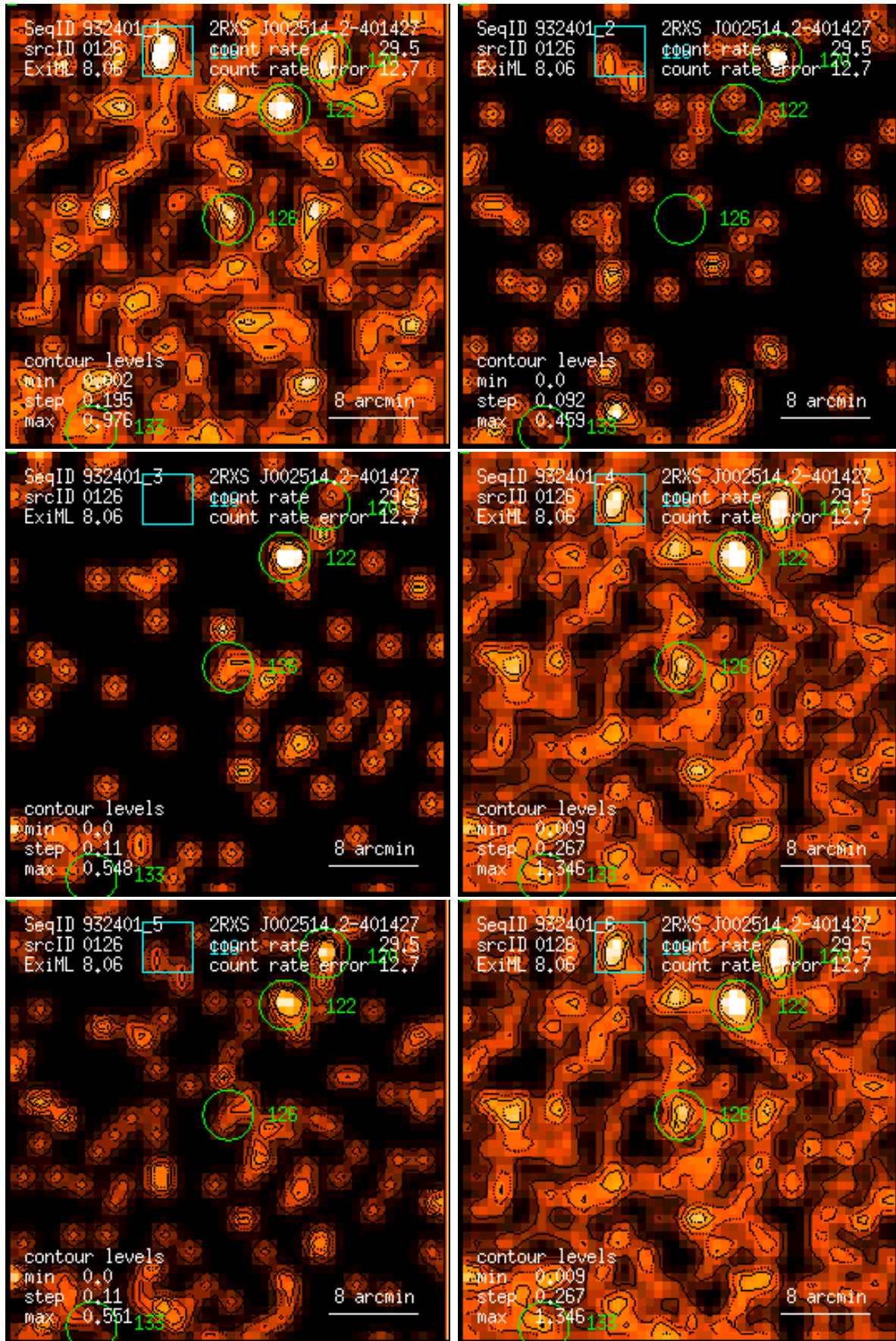
Figure 126: RASS 932401: detection 0126: band rate images, Gaussian filter: (1) PSPPC channels 11 – 41, (2) 52 – 90, (3) 91 – 201, (4) 11 – 235, (5) 52 – 201, (6) 11 – 201. Broad band rates in counts/ks. Band rate contour levels in counts/ks/arcmin 2 .
