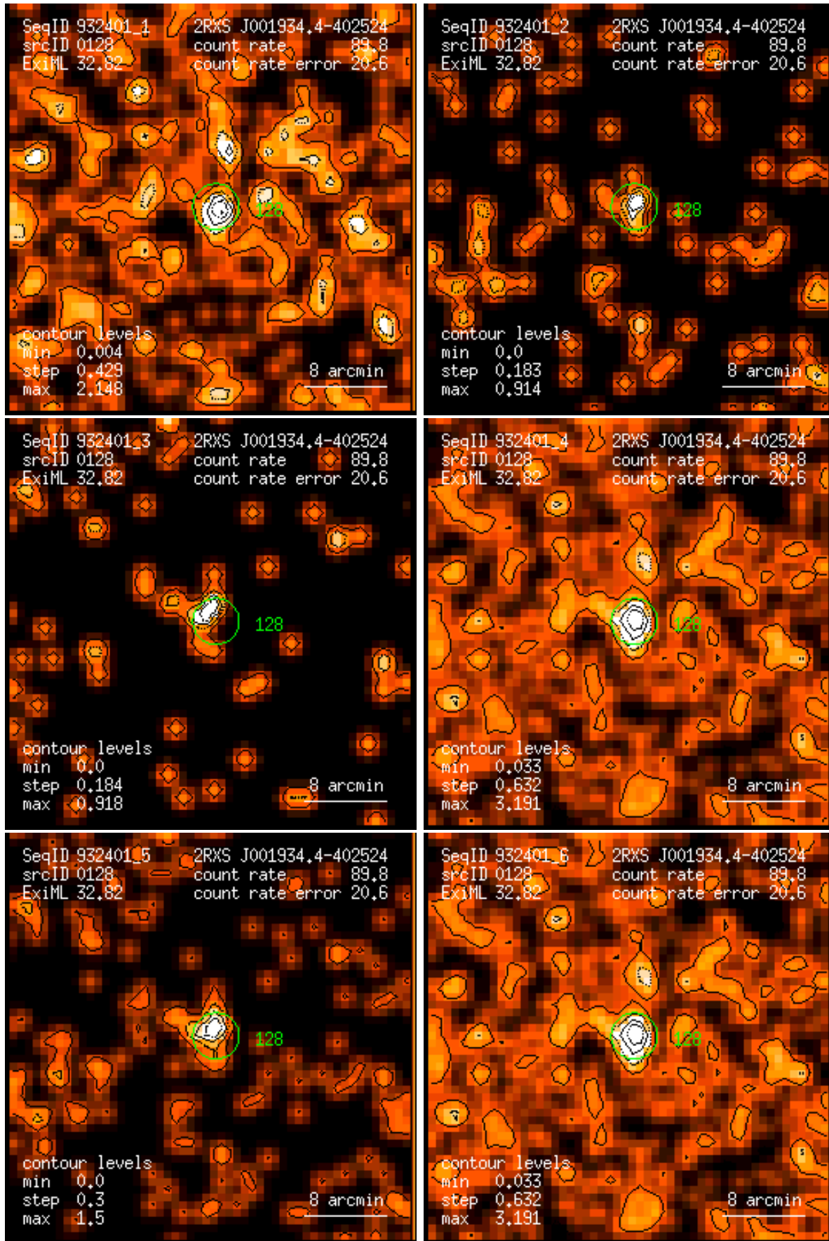
Figure 128: RASS 932401: detection 0128: band rate images, Gaussian filter: (1) PSPC channels 11 – 41, (2) 52 – 90, (3) 91 – 201, (4) 11 – 235, (5) 52 – 201, (6) 11 – 201. Broad band rates in counts/ks. Band rate contour levels in counts/ks/arcmin 2 .
