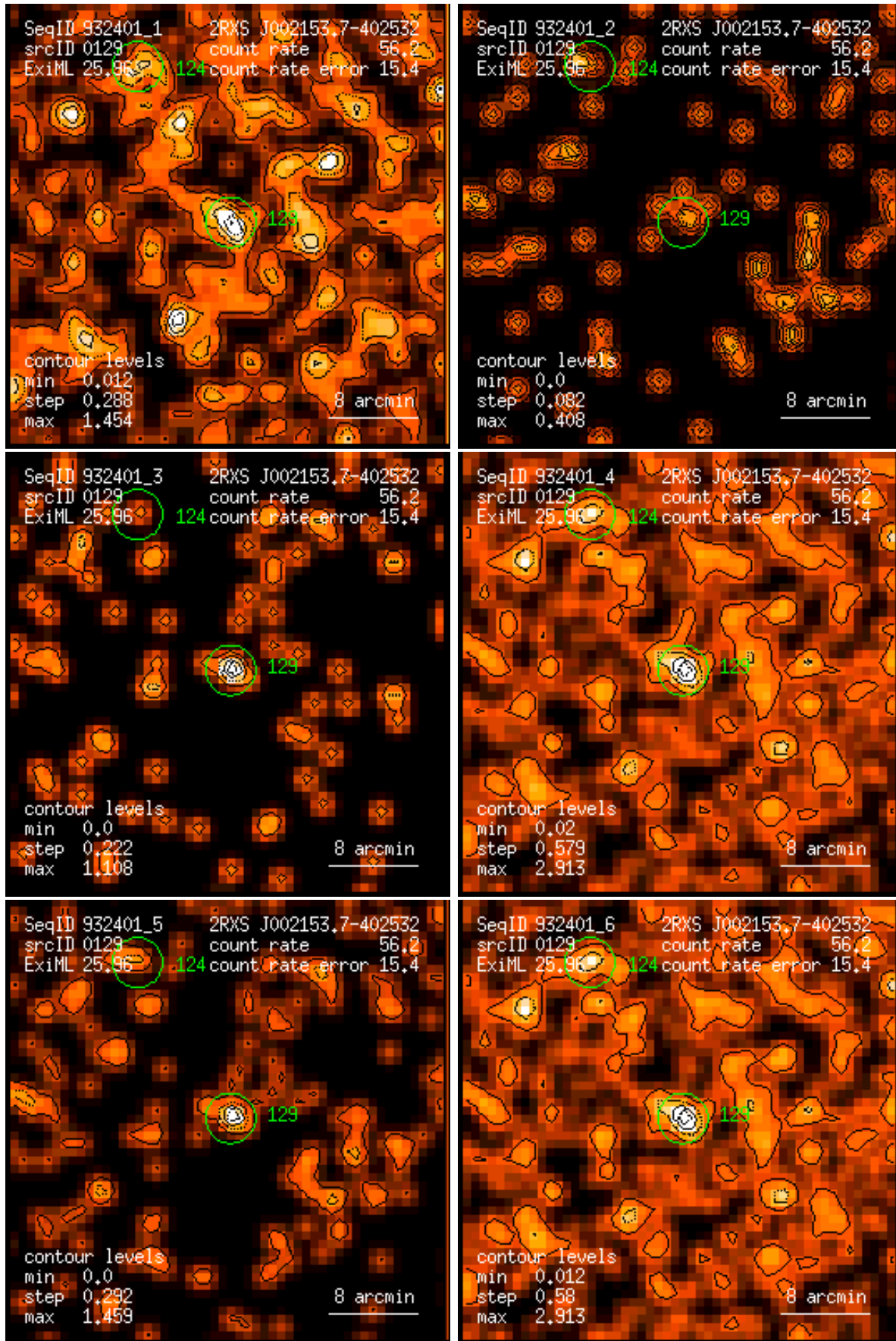
Figure 129: RASS 932401: detection 0129: band rate images, Gaussian filter: (1) PSPC channels 11 – 41, (2) 52 – 90, (3) 91 – 201, (4) 11 – 235, (5) 52 – 201, (6) 11 – 201. Broad band rates in counts/ks. Band rate contour levels in counts/ks/arcmin 2 .
