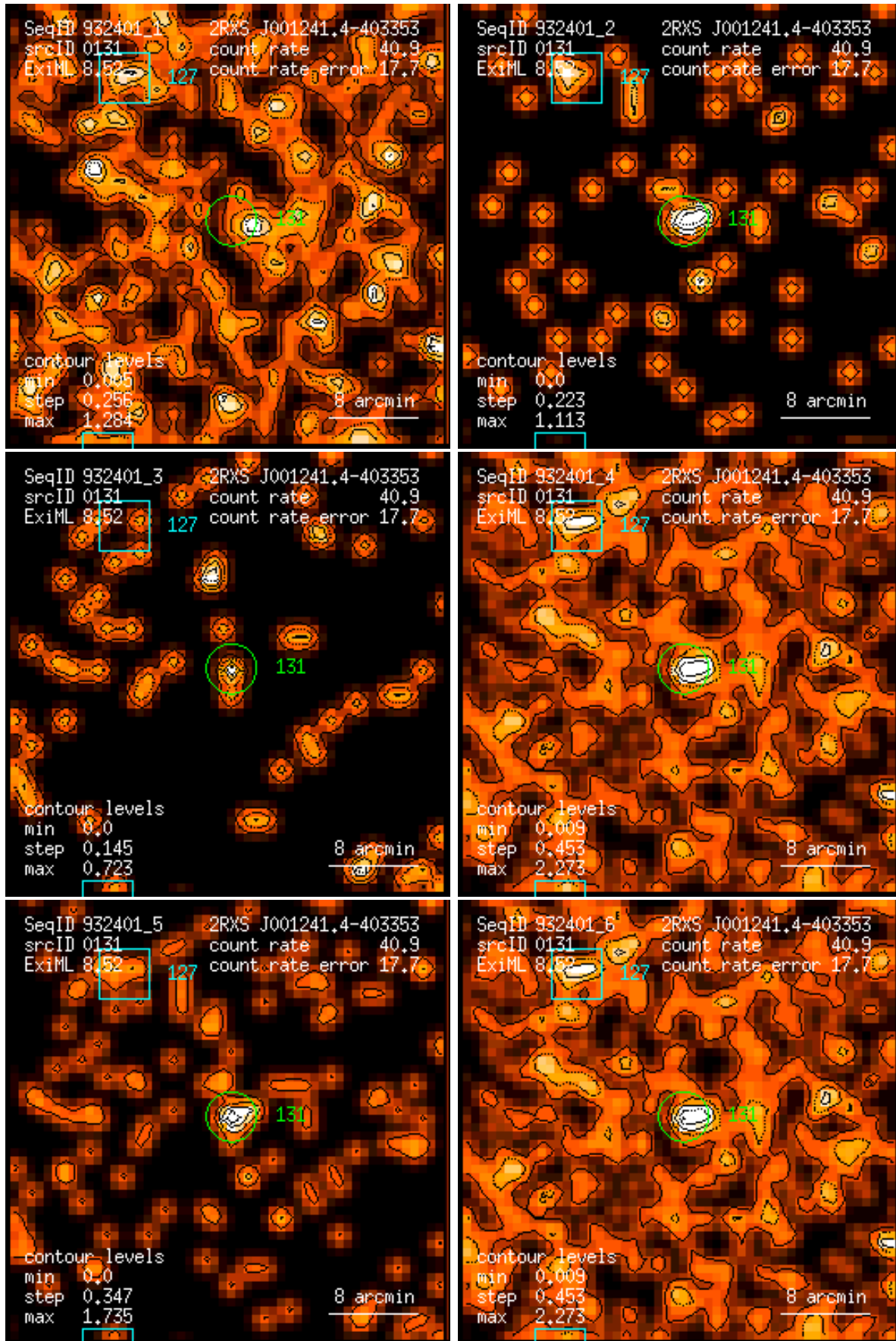
Figure 131: RASS 932401: detection 0131: band rate images, Gaussian filter: (1) PSPC channels 11 – 41, (2) 52 – 90, (3) 91 – 201, (4) 11 – 235, (5) 52 – 201, (6) 11 – 201. Broad band rates in counts/ks. Band rate contour levels in counts/ks/arcmin 2 .
