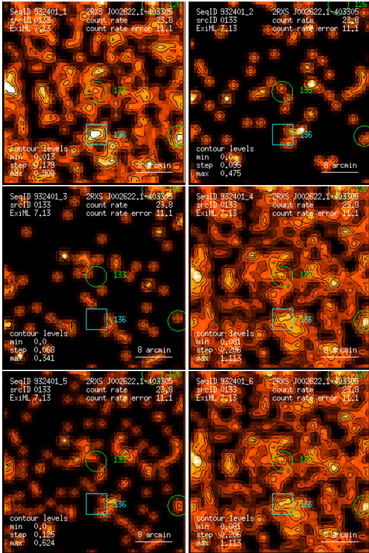
Figure 133: RASS 932401: detection 0133: band rate images, Gaussian filter: (1) PSPC channels 11 – 41, (2) 52 – 90, (3) 91 – 201, (4) 11 – 235, (5) 52 – 201, (6) 11 – 201. Broad band rates in counts/ks. Band rate contour levels in counts/ks/arcmin 2 .
