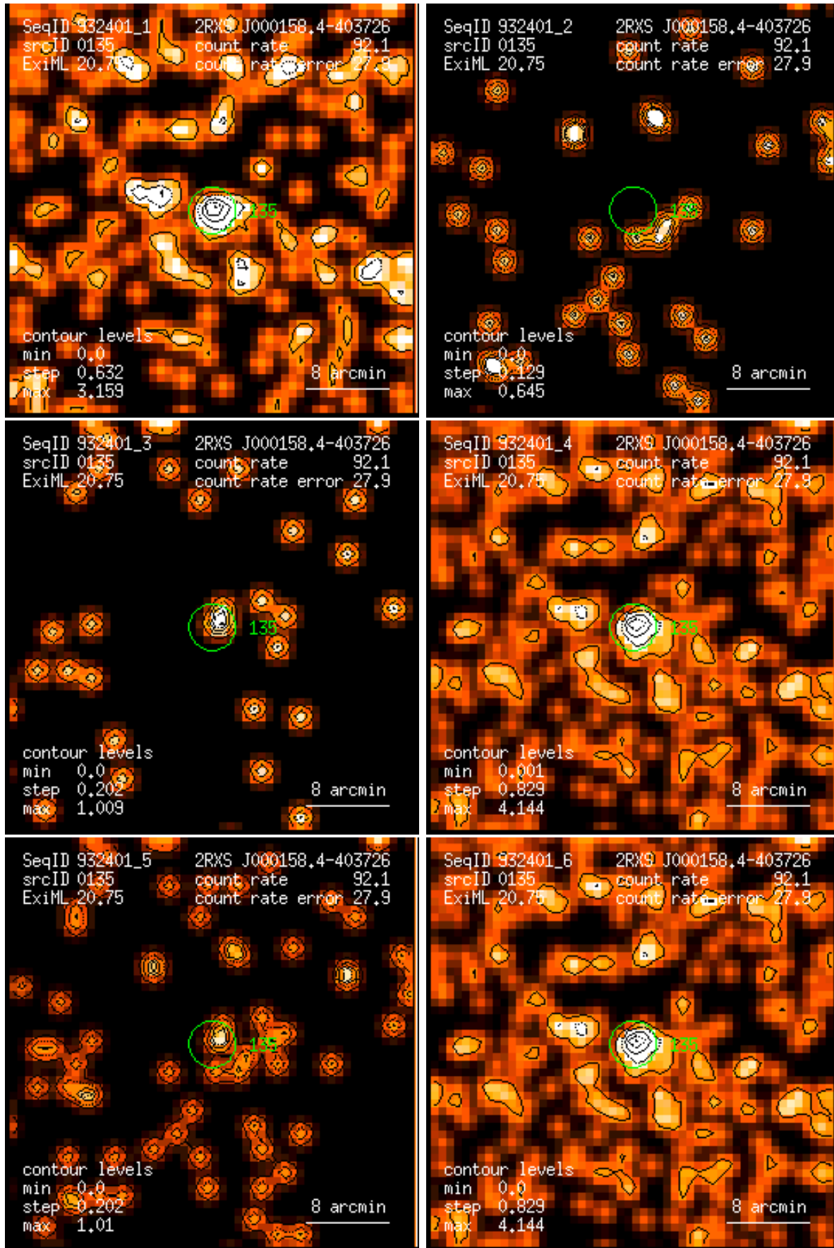
Figure 135: RASS 932401: detection 0135: band rate images, Gaussian filter: (1) PSPC channels 11 – 41, (2) 52 – 90, (3) 91 – 201, (4) 11 – 235, (5) 52 – 201, (6) 11 – 201. Broad band rates in counts/ks. Band rate contour levels in counts/ks/arcmin 2 .
