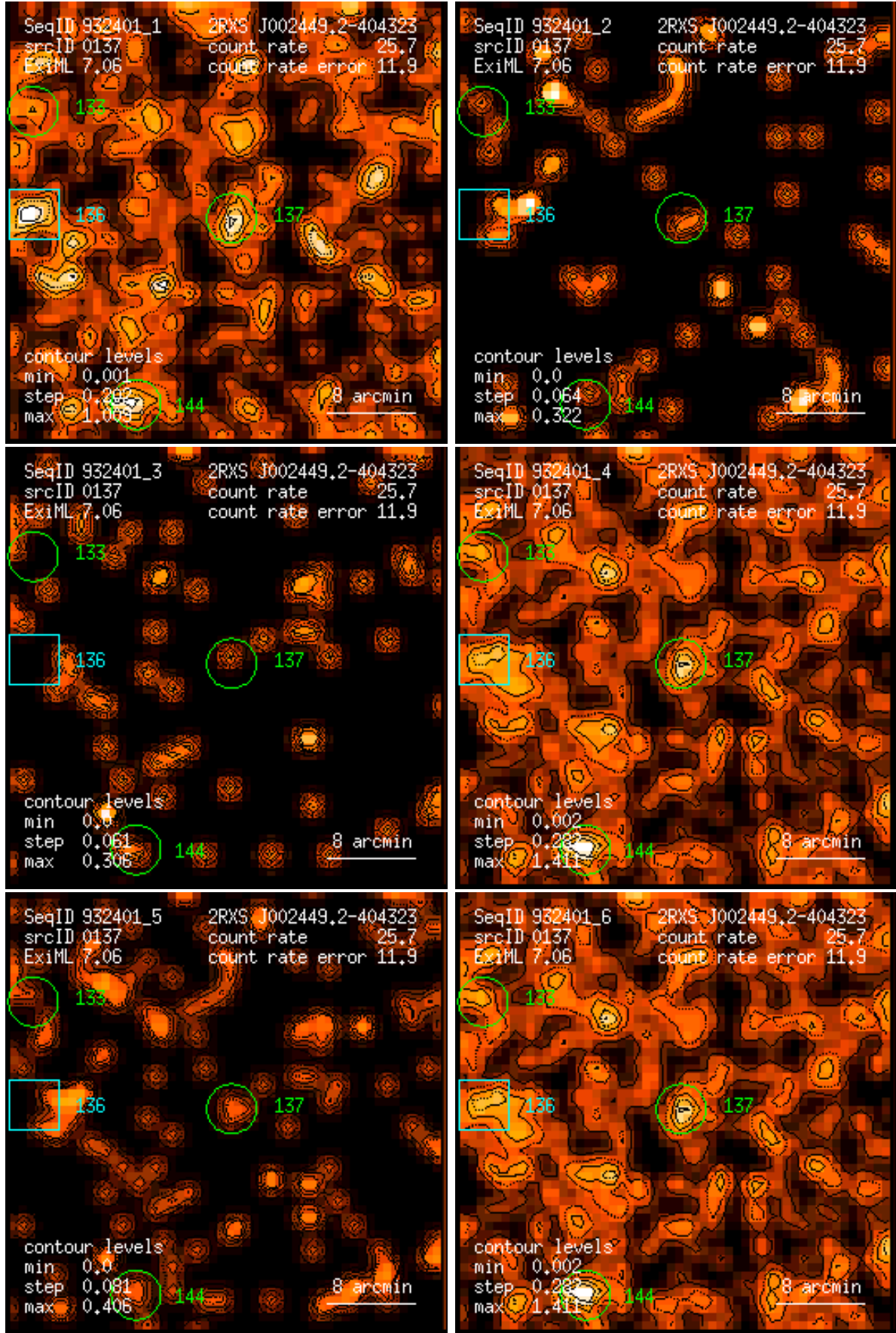
Figure 137: RASS 932401: detection 0137: band rate images, Gaussian filter: (1) PSPC channels 11 – 41, (2) 52 – 90, (3) 91 – 201, (4) 11 – 235, (5) 52 – 201, (6) 11 – 201. Broad band rates in counts/ks. Band rate contour levels in counts/ks/arcmin 2 .
