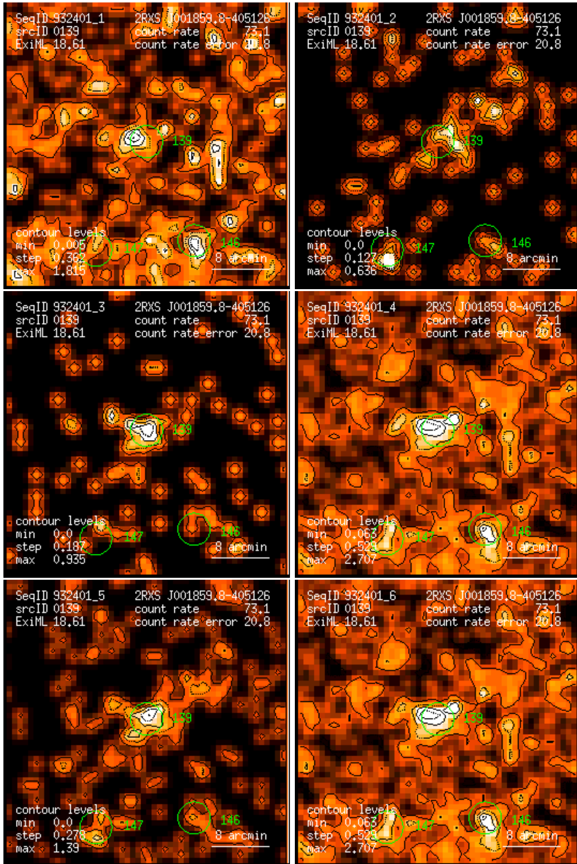
Figure 139: RASS 932401: detection 0139: band rate images, Gaussian filter: (1) PSPC channels 11 – 41, (2) 52 – 90, (3) 91 – 201, (4) 11 – 235, (5) 52 – 201, (6) 11 – 201. Broad band rates in counts/ks. Band rate contour levels in counts/ks/arcmin 2 .
