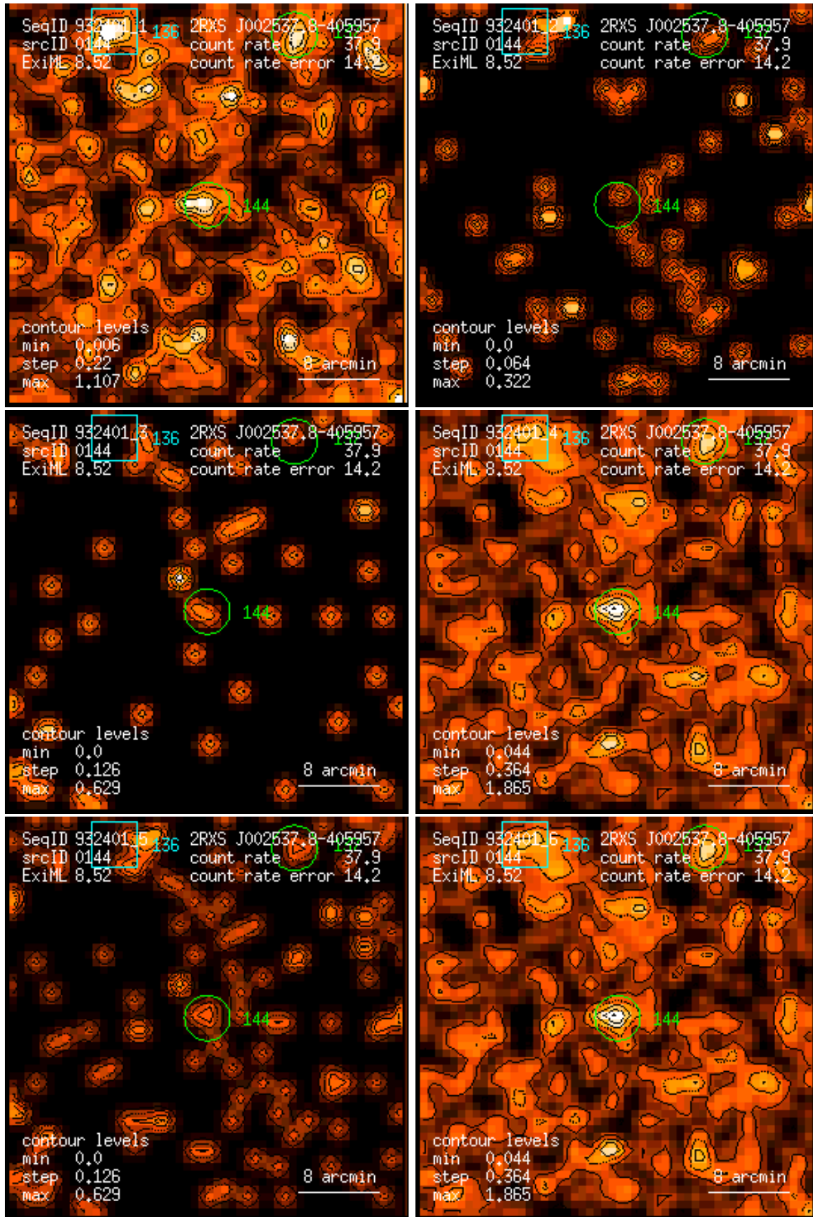
Figure 144: RASS 932401: detection 0144: band rate images, Gaussian filter: (1) PSPC channels 11 – 41, (2) 52 – 90, (3) 91 – 201, (4) 11 – 235, (5) 52 – 201, (6) 11 – 201. Broad band rates in counts/ks. Band rate contour levels in counts/ks/arcmin 2 .
