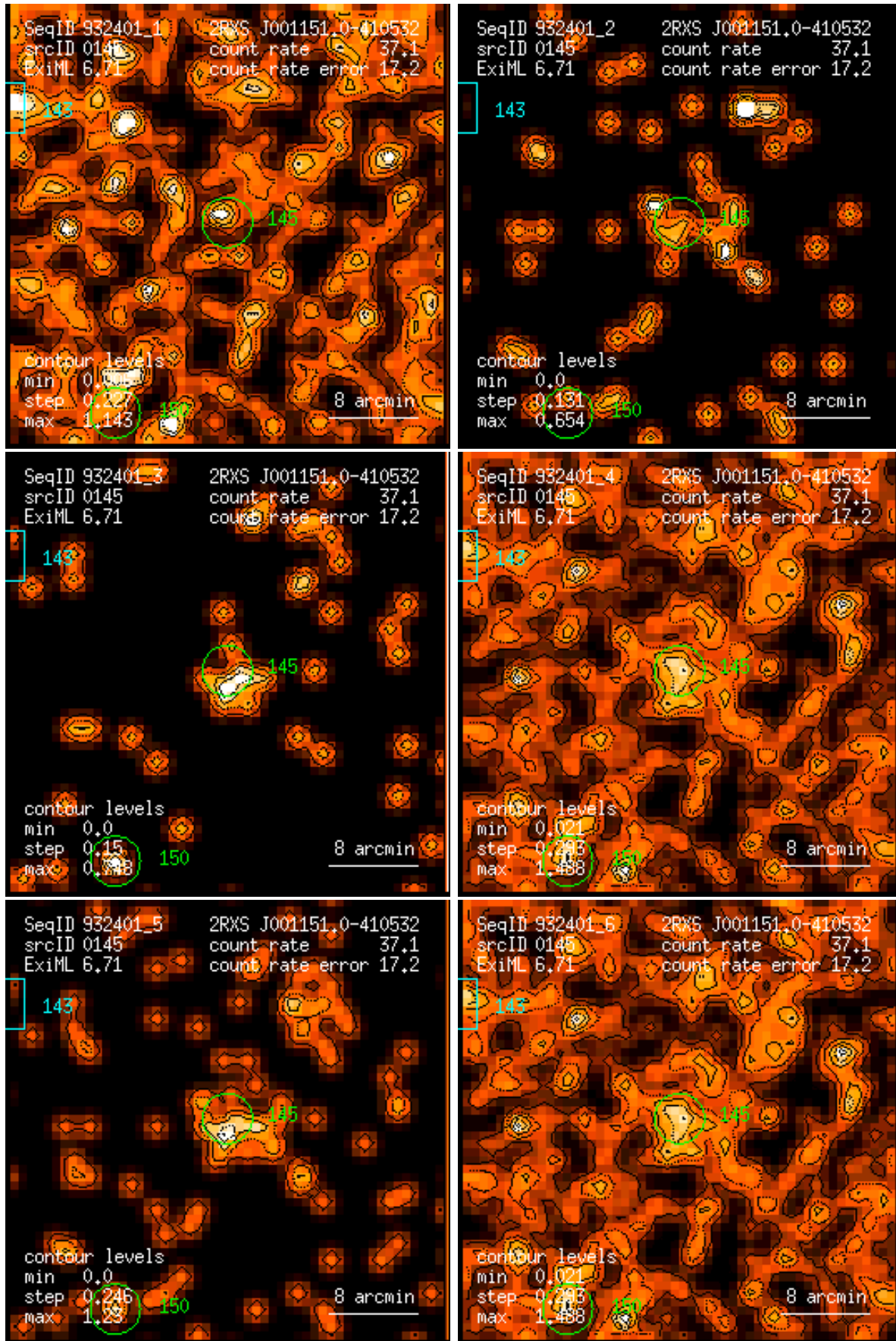
Figure 145: RASS 932401: detection 0145: band rate images, Gaussian filter: (1) PSPC channels 11 – 41, (2) 52 – 90, (3) 91 – 201, (4) 11 – 235, (5) 52 – 201, (6) 11 – 201. Broad band rates in counts/ks. Band rate contour levels in counts/ks/arcmin 2 .
