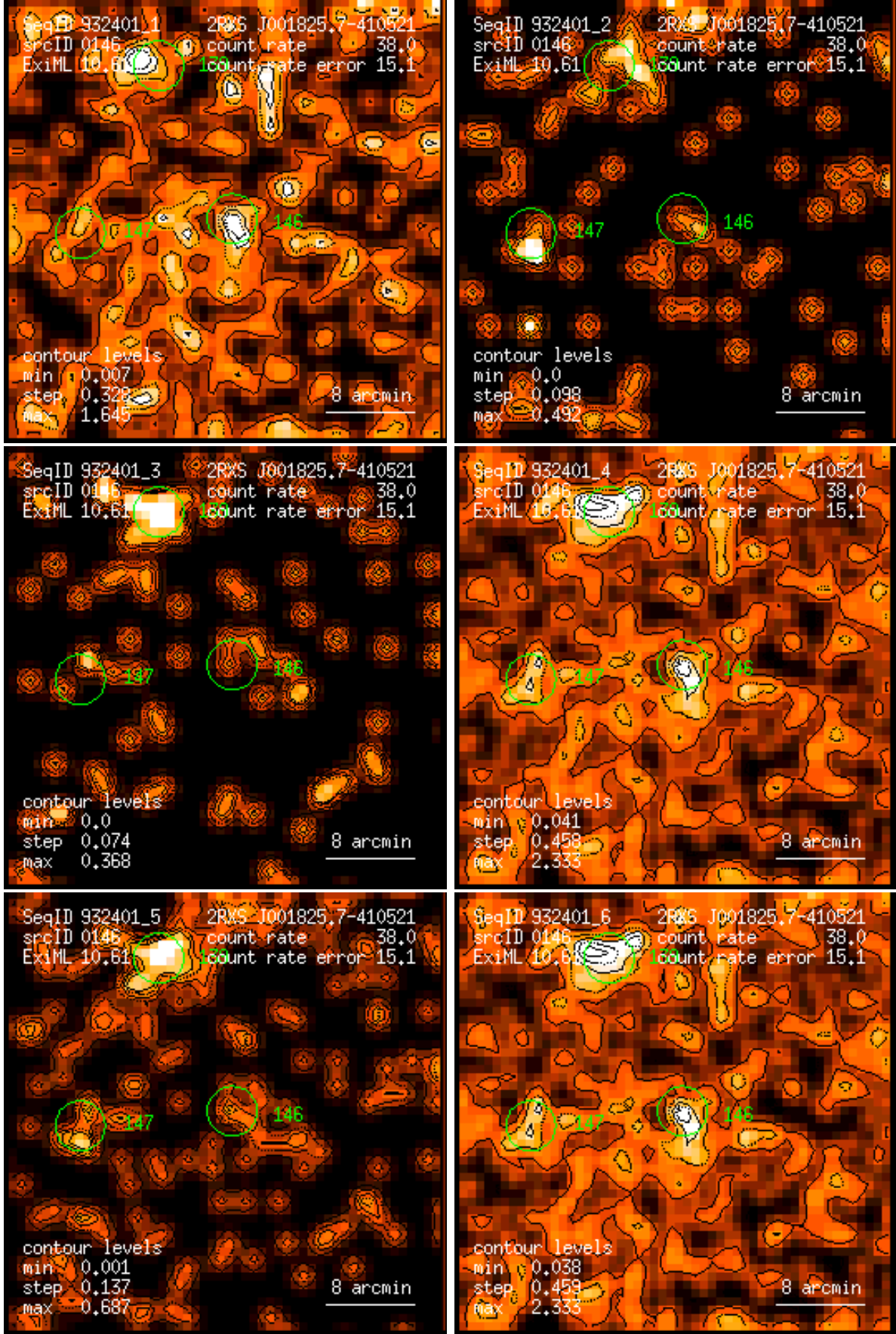
Figure 146: RASS 932401: detection 0146: band rate images, Gaussian filter: (1) PSPC channels 11 – 41, (2) 52 – 90, (3) 91 – 201, (4) 11 – 235, (5) 52 – 201, (6) 11 – 201. Broad band rates in counts/ks. Band rate contour levels in counts/ks/arcmin 2 .
