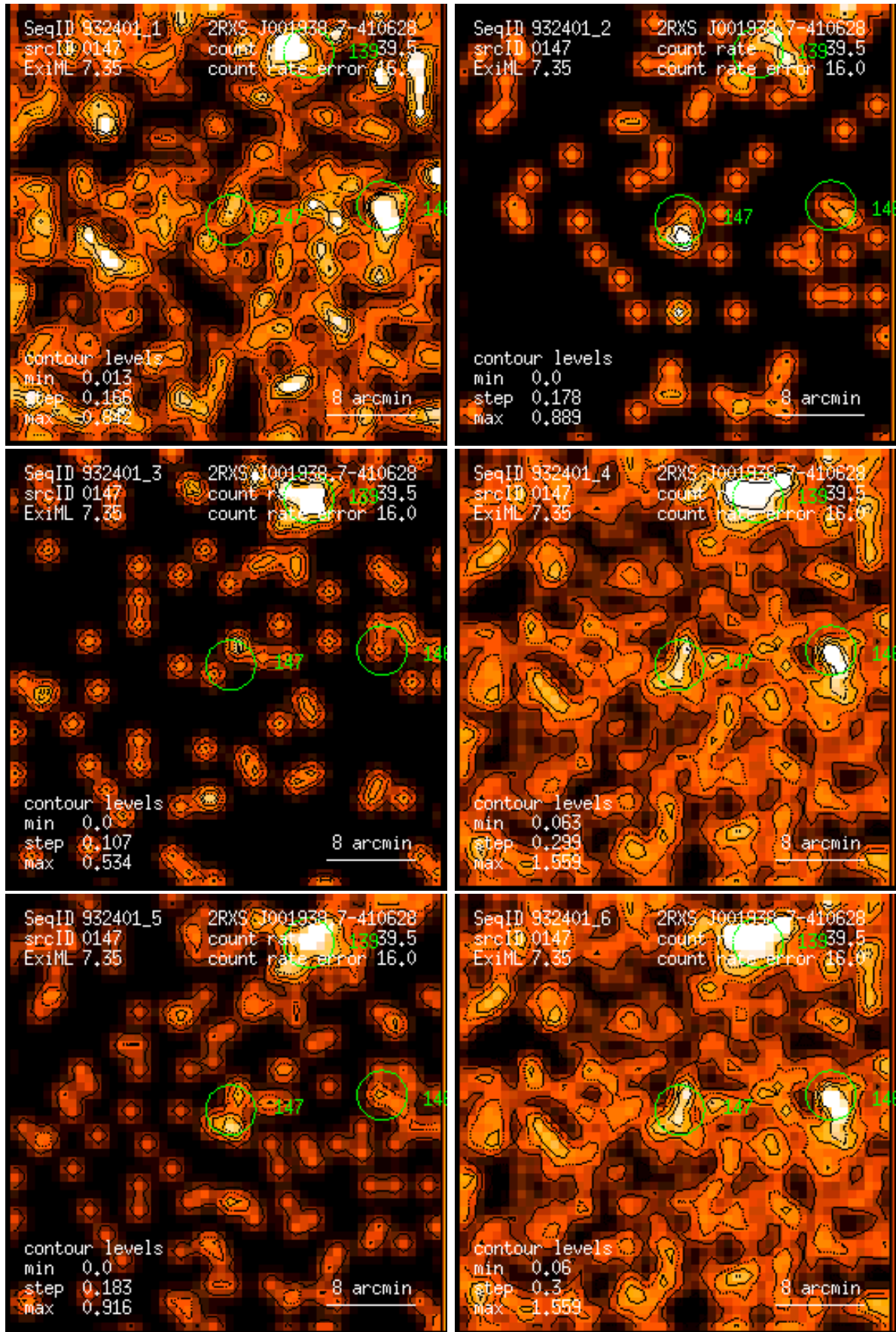
Figure 147: RASS 932401: detection 0147: band rate images, Gaussian filter: (1) PSPC channels 11 – 41, (2) 52 – 90, (3) 91 – 201, (4) 11 – 235, (5) 52 – 201, (6) 11 – 201. Broad band rates in counts/ks. Band rate contour levels in counts/ks/arcmin 2 .
