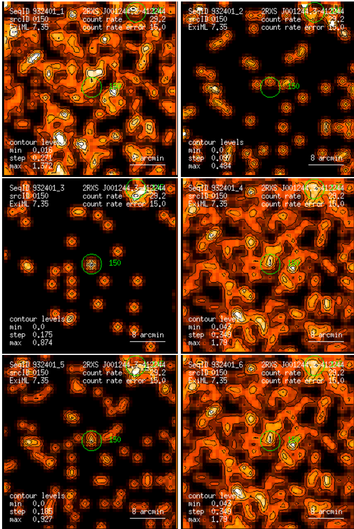
Figure 150: RASS 932401: detection 0150: band rate images, Gaussian filter: (1) PSPC channels 11 – 41, (2) 52 – 90, (3) 91 – 201, (4) 11 – 235, (5) 52 – 201, (6) 11 – 201. Broad band rates in counts/ks. Band rate contour levels in counts/ks/arcmin 2 .
