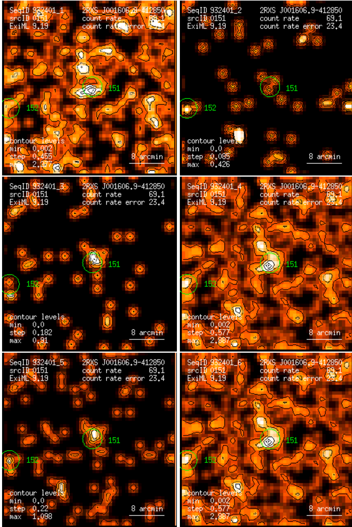
Figure 151: RASS 932401: detection 0151: band rate images, Gaussian filter: (1) PSPC channels 11 – 41, (2) 52 – 90, (3) 91 – 201, (4) 11 – 235, (5) 52 – 201, (6) 11 – 201. Broad band rates in counts/ks. Band rate contour levels in counts/ks/arcmin 2 .
