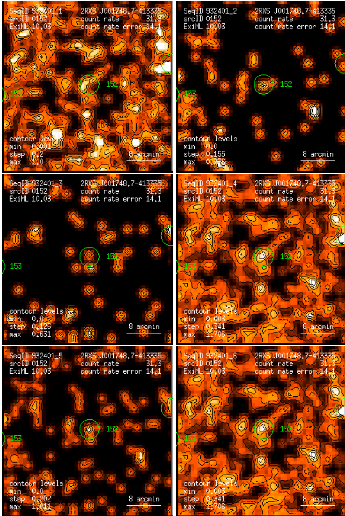
Figure 152: RASS 932401: detection 0152: band rate images, Gaussian filter: (1) PSPC channels 11 – 41, (2) 52 – 90, (3) 91 – 201, (4) 11 – 235, (5) 52 – 201, (6) 11 – 201. Broad band rates in counts/ks. Band rate contour levels in counts/ks/arcmin 2 .
