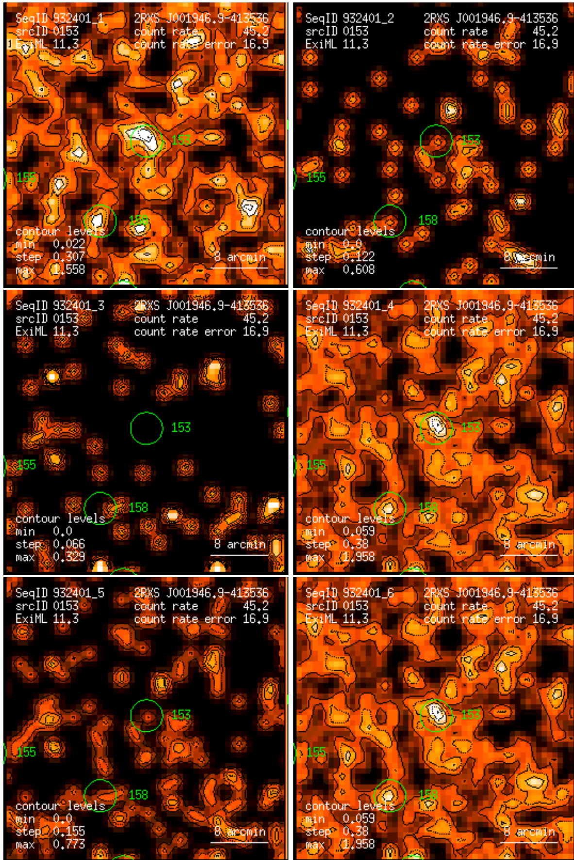
Figure 153: RASS 932401: detection 0153: band rate images, Gaussian filter: (1) PSPC channels 11 – 41, (2) 52 – 90, (3) 91 – 201, (4) 11 – 235, (5) 52 – 201, (6) 11 – 201. Broad band rates in counts/ks. Band rate contour levels in counts/ks/arcmin 2 .
