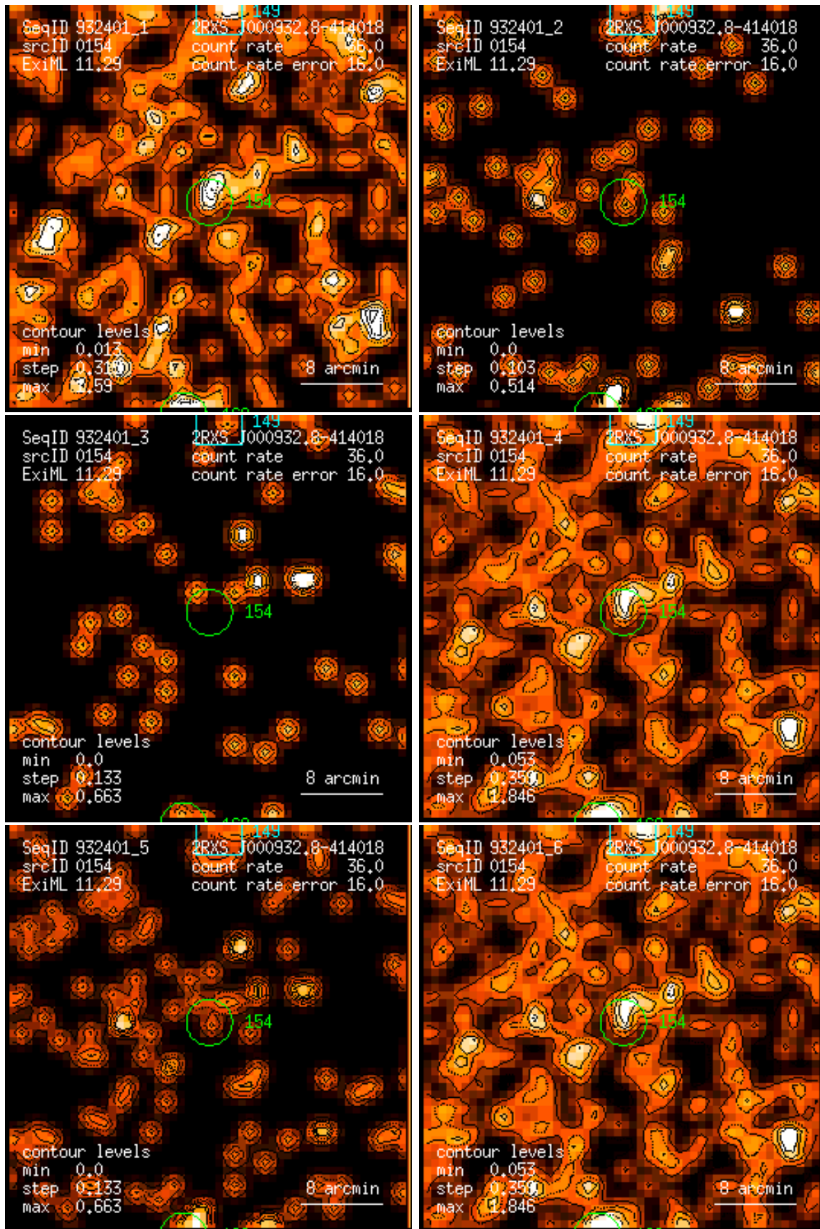
Figure 154: RASS 932401: detection 0154: band rate images, Gaussian filter: (1) PSPC channels 11 – 41, (2) 52 – 90, (3) 91 – 201, (4) 11 – 235, (5) 52 – 201, (6) 11 – 201. Broad band rates in counts/ks. Band rate contour levels in counts/ks/arcmin 2 .
