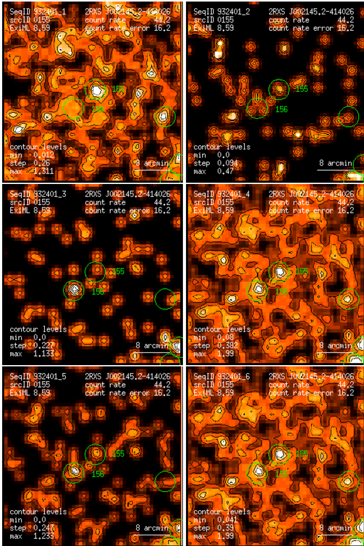
Figure 155: RASS 932401: detection 0155: band rate images, Gaussian filter: (1) PSPC channels 11 – 41, (2) 52 – 90, (3) 91 – 201, (4) 11 – 235, (5) 52 – 201, (6) 11 – 201. Broad band rates in counts/ks. Band rate contour levels in counts/ks/arcmin 2 .
