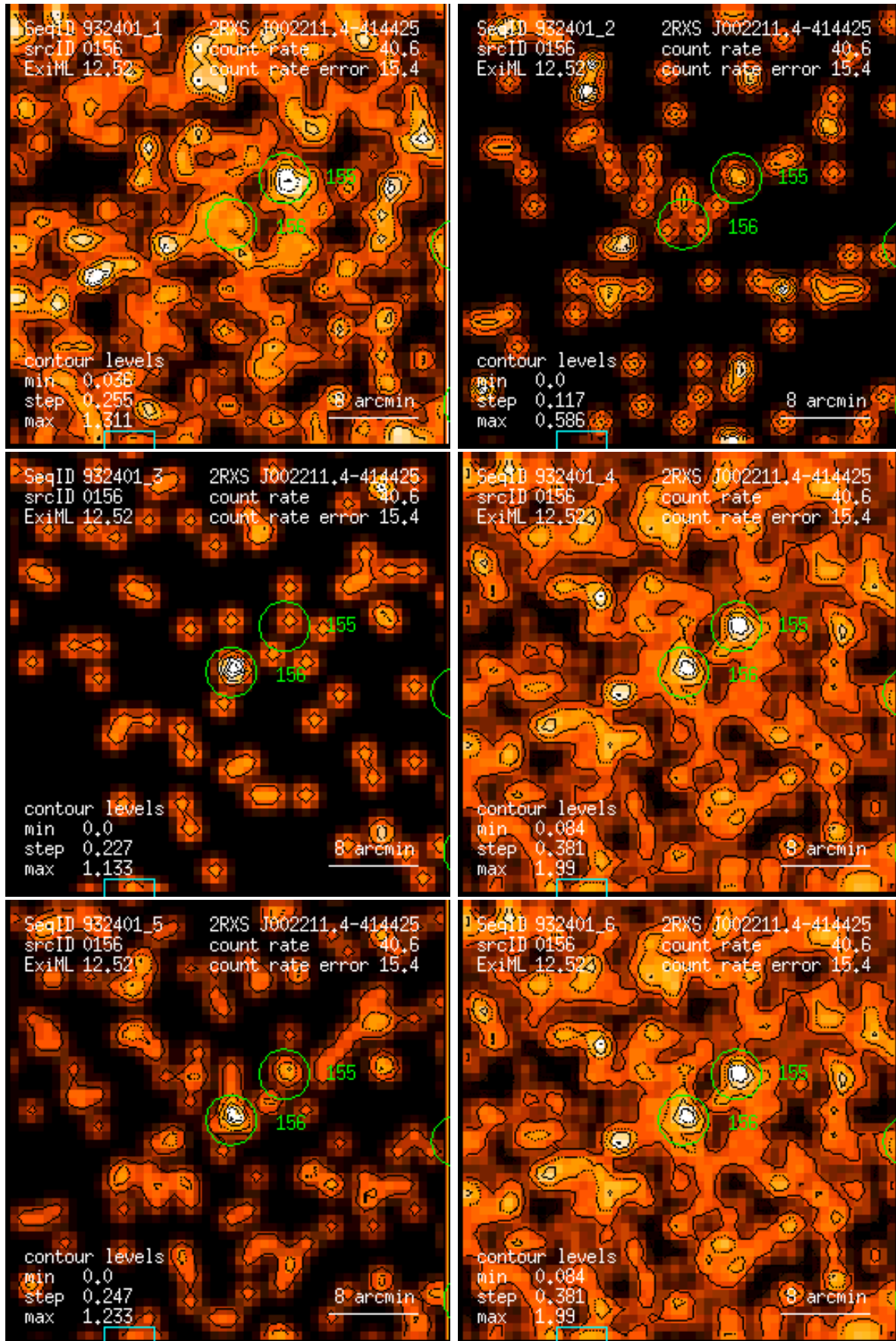
Figure 156: RASS 932401: detection 0156: band rate images, Gaussian filter: (1) PSPC channels 11 – 41, (2) 52 – 90, (3) 91 – 201, (4) 11 – 235, (5) 52 – 201, (6) 11 – 201. Broad band rates in counts/ks. Band rate contour levels in counts/ks/arcmin 2 .
