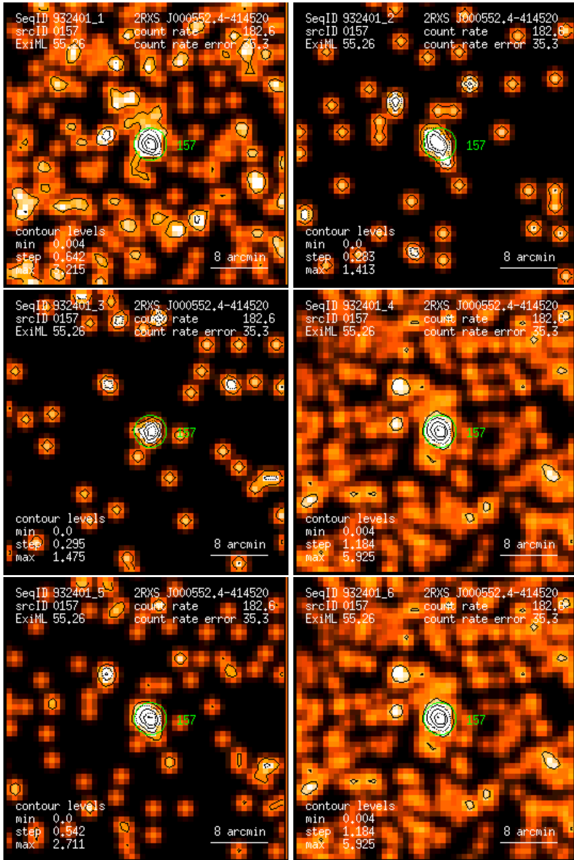
Figure 157: RASS 932401: detection 0157: band rate images, Gaussian filter: (1) PSPC channels 11 – 41, (2) 52 – 90, (3) 91 – 201, (4) 11 – 235, (5) 52 – 201, (6) 11 – 201. Broad band rates in counts/ks. Band rate contour levels in counts/ks/arcmin 2 .
