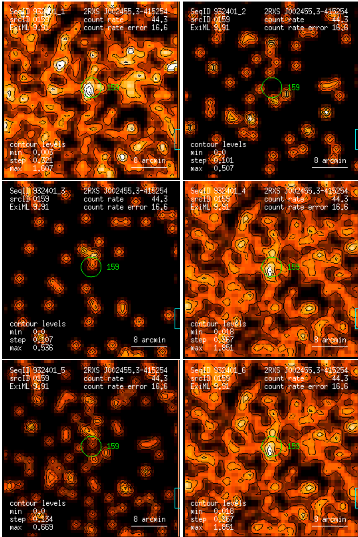
Figure 159: RASS 932401: detection 0159: band rate images, Gaussian filter: (1) PSPC channels 11 – 41, (2) 52 – 90, (3) 91 – 201, (4) 11 – 235, (5) 52 – 201, (6) 11 – 201. Broad band rates in counts/ks. Band rate contour levels in counts/ks/arcmin 2 .
