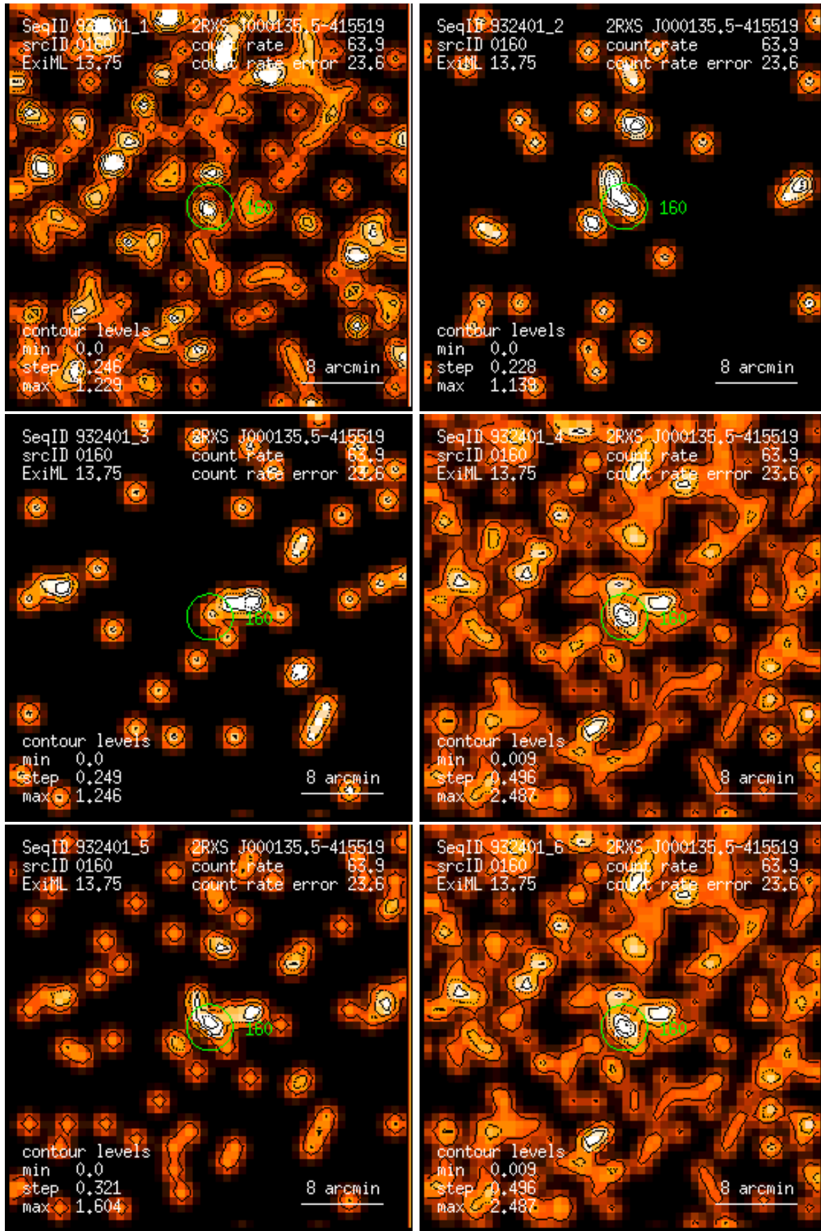
Figure 160: RASS 932401: detection 0160: band rate images, Gaussian filter: (1) PSPC channels 11 – 41, (2) 52 – 90, (3) 91 – 201, (4) 11 – 235, (5) 52 – 201, (6) 11 – 201. Broad band rates in counts/ks. Band rate contour levels in counts/ks/arcmin 2 .
