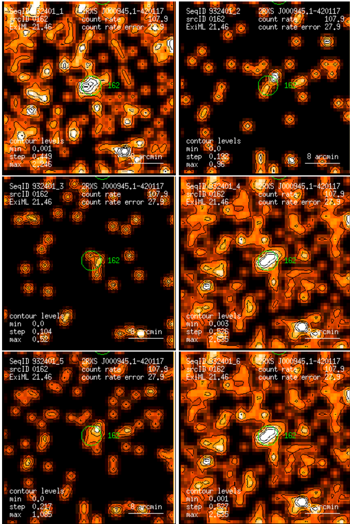
Figure 162: RASS 932401: detection 0162: band rate images, Gaussian filter: (1) PSPC channels 11 – 41, (2) 52 – 90, (3) 91 – 201, (4) 11 – 235, (5) 52 – 201, (6) 11 – 201. Broad band rates in counts/ks. Band rate contour levels in counts/ks/arcmin 2 .
