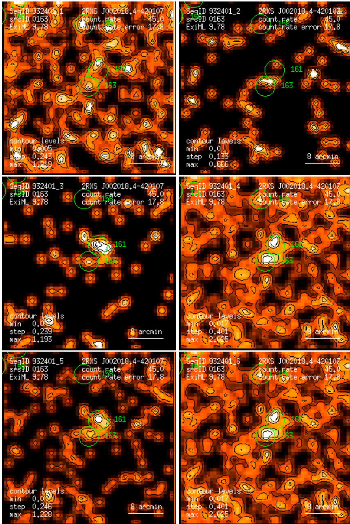
Figure 163: RASS 932401: detection 0163: band rate images, Gaussian filter: (1) PSPC channels 11 – 41, (2) 52 – 90, (3) 91 – 201, (4) 11 – 235, (5) 52 – 201, (6) 11 – 201. Broad band rates in counts/ks. Band rate contour levels in counts/ks/arcmin 2 .
