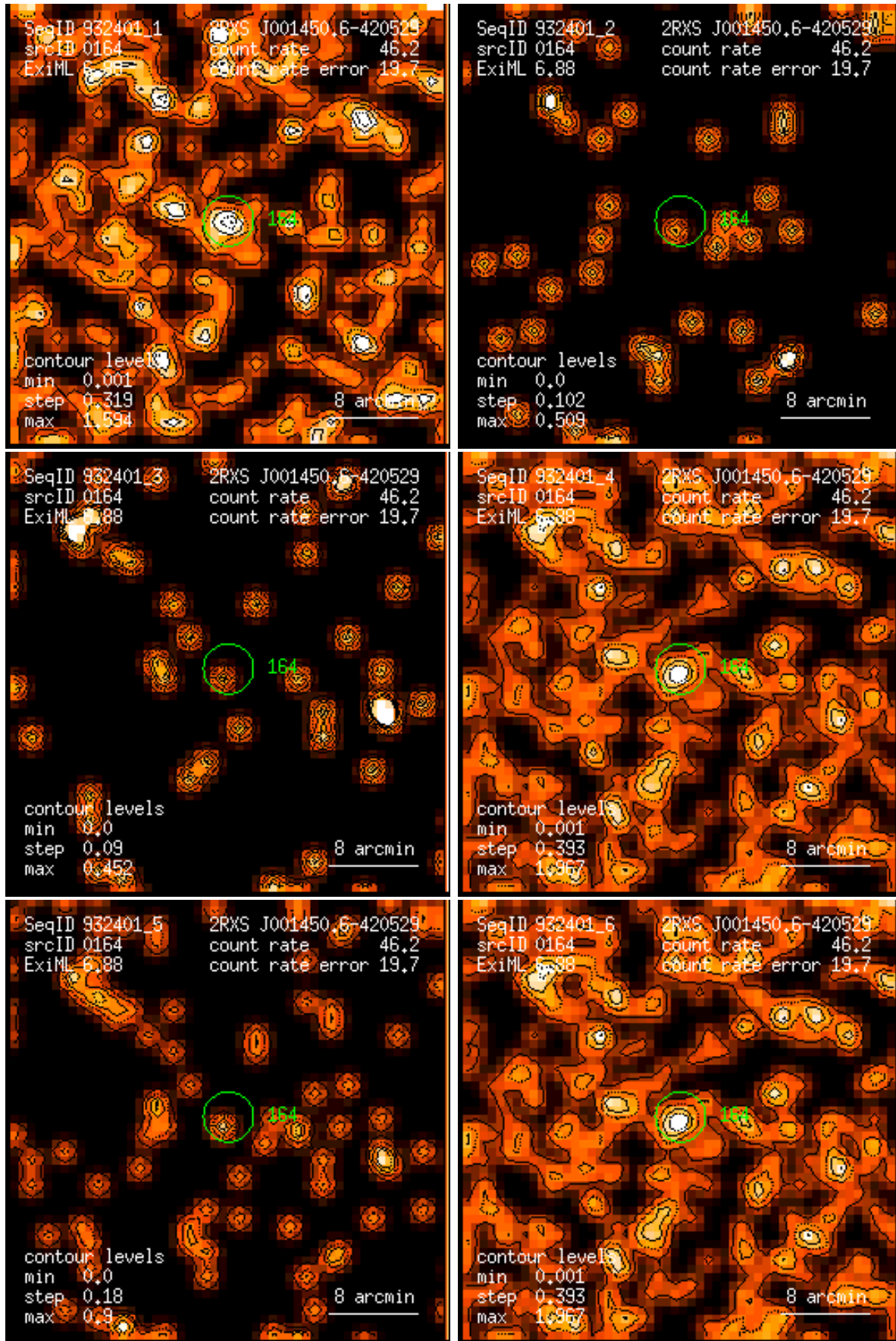
Figure 164: RASS 932401: detection 0164: band rate images, Gaussian filter: (1) PSPC channels 11 – 41, (2) 52 – 90, (3) 91 – 201, (4) 11 – 235, (5) 52 – 201, (6) 11 – 201. Broad band rates in counts/ks. Band rate contour levels in counts/ks/arcmin 2 .
