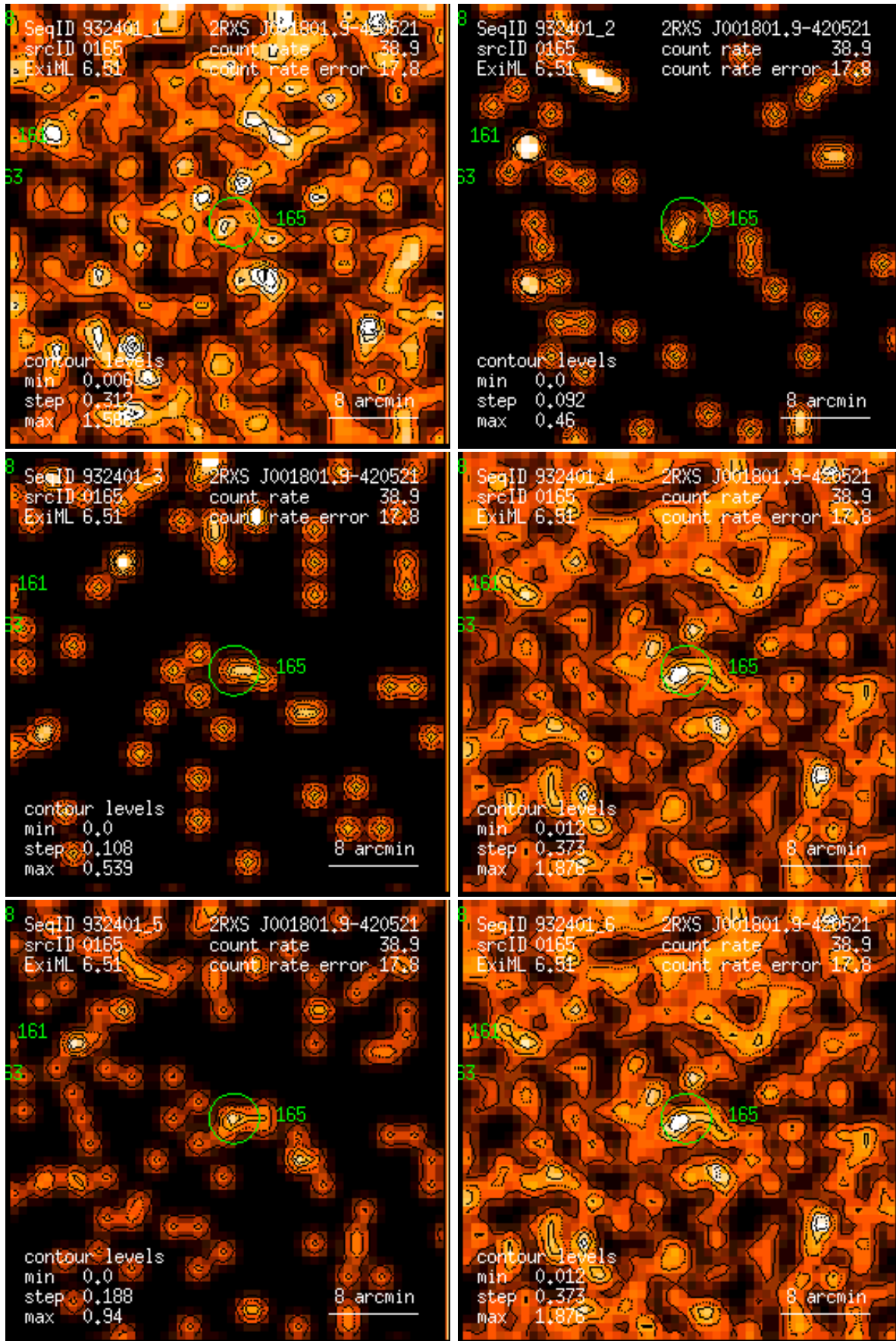
Figure 165: RASS 932401: detection 0165: band rate images, Gaussian filter: (1) PSPC channels 11 – 41, (2) 52 – 90, (3) 91 – 201, (4) 11 – 235, (5) 52 – 201, (6) 11 – 201. Broad band rates in counts/ks. Band rate contour levels in counts/ks/arcmin 2 .
