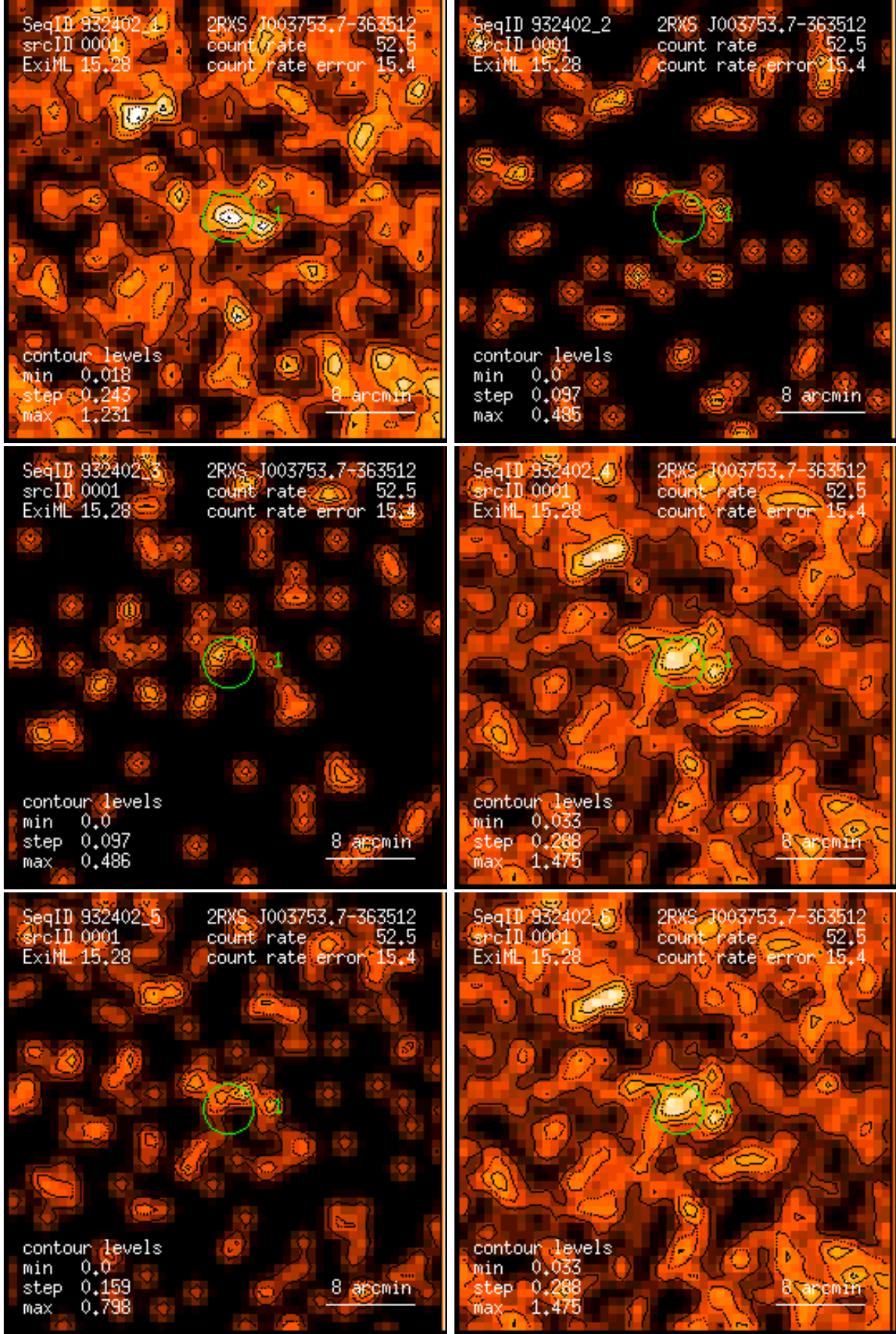
Figure 1: RASS 932402: detection 0001: band rate images, Gaussian filter: (1) PSPC channels 11 – 41, (2) 52 – 90, (3) 91 – 201, (4) 11 – 235, (5) 52 – 201, (6) 11 – 201. Broad band rates in counts/ks. Band rate contour levels in counts/ks/arcmin 2 .
