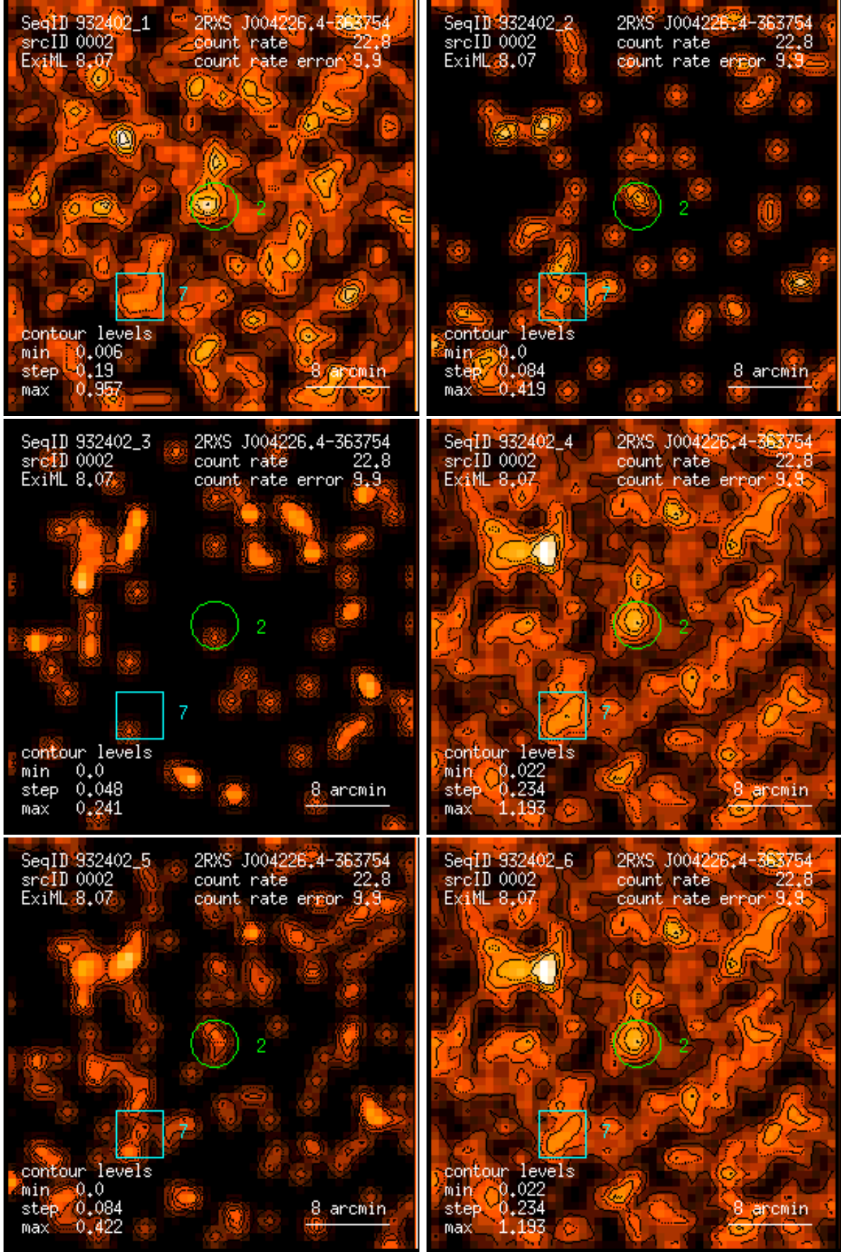
Figure 2: RASS 932402: detection 0002: band rate images, Gaussian filter: (1) PSPC channels 11 – 41, (2) 52 – 90, (3) 91 – 201, (4) 11 – 235, (5) 52 – 201, (6) 11 – 201. Broad band rates in counts/ks. Band rate contour levels in counts/ks/arcmin 2 .
