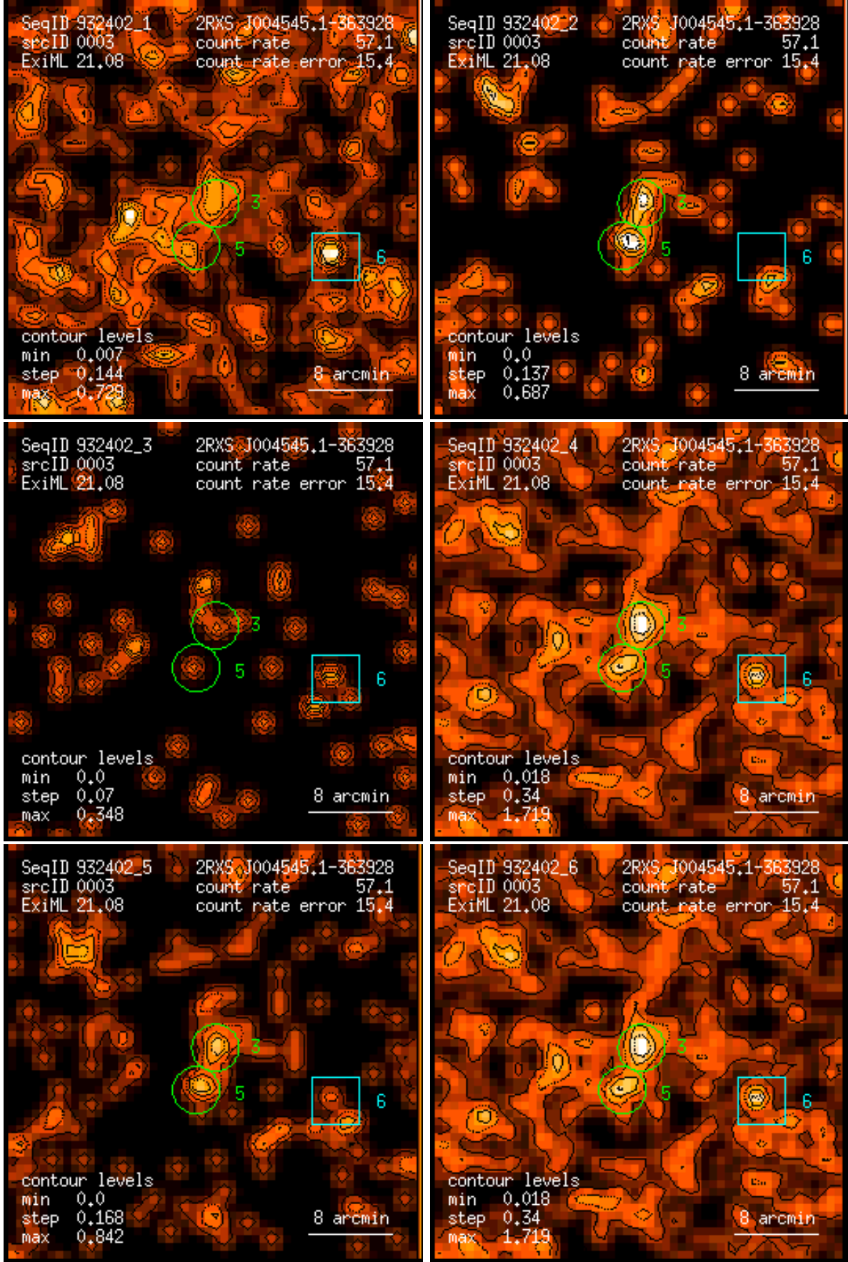
Figure 3: RASS 932402: detection 0003: band rate images, Gaussian filter: (1) PSPC channels 11 – 41, (2) 52 – 90, (3) 91 – 201, (4) 11 – 235, (5) 52 – 201, (6) 11 – 201. Broad band rates in counts/ks. Band rate contour levels in counts/ks/arcmin 2 .
