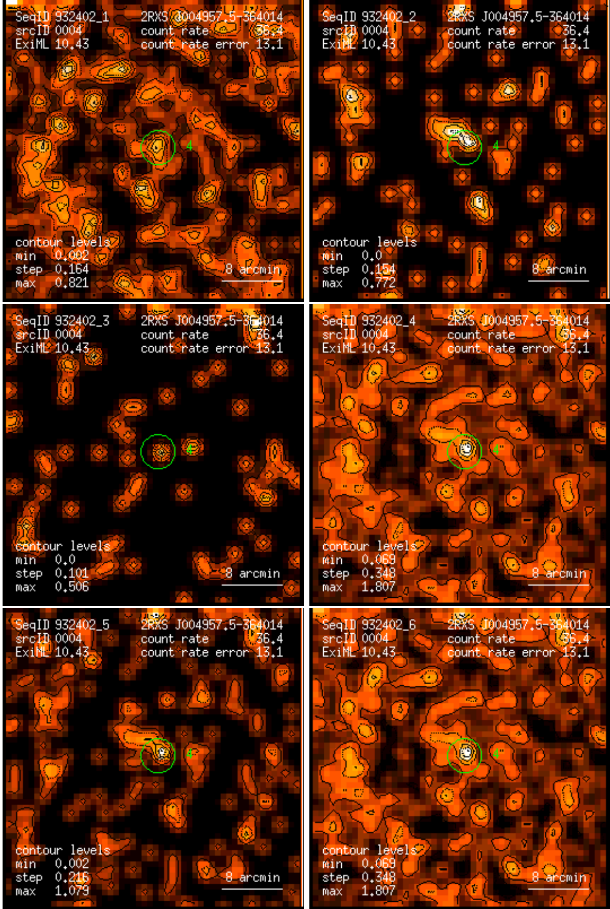
Figure 4: RASS 932402: detection 0004: band rate images, Gaussian filter: (1) PSPC channels 11 – 41, (2) 52 – 90, (3) 91 – 201, (4) 11 – 235, (5) 52 – 201, (6) 11 – 201. Broad band rates in counts/ks. Band rate contour levels in counts/ks/arcmin 2 .
