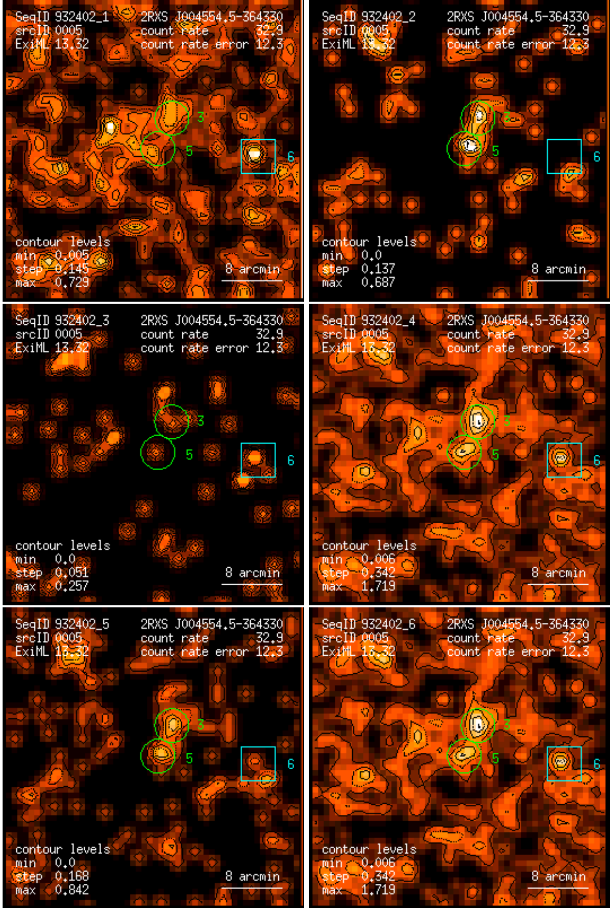
Figure 5: RASS 932402: detection 0005: band rate images, Gaussian filter: (1) PSPC channels 11 – 41, (2) 52 – 90, (3) 91 – 201, (4) 11 – 235, (5) 52 – 201, (6) 11 – 201. Broad band rates in counts/ks. Band rate contour levels in counts/ks/arcmin 2 .
