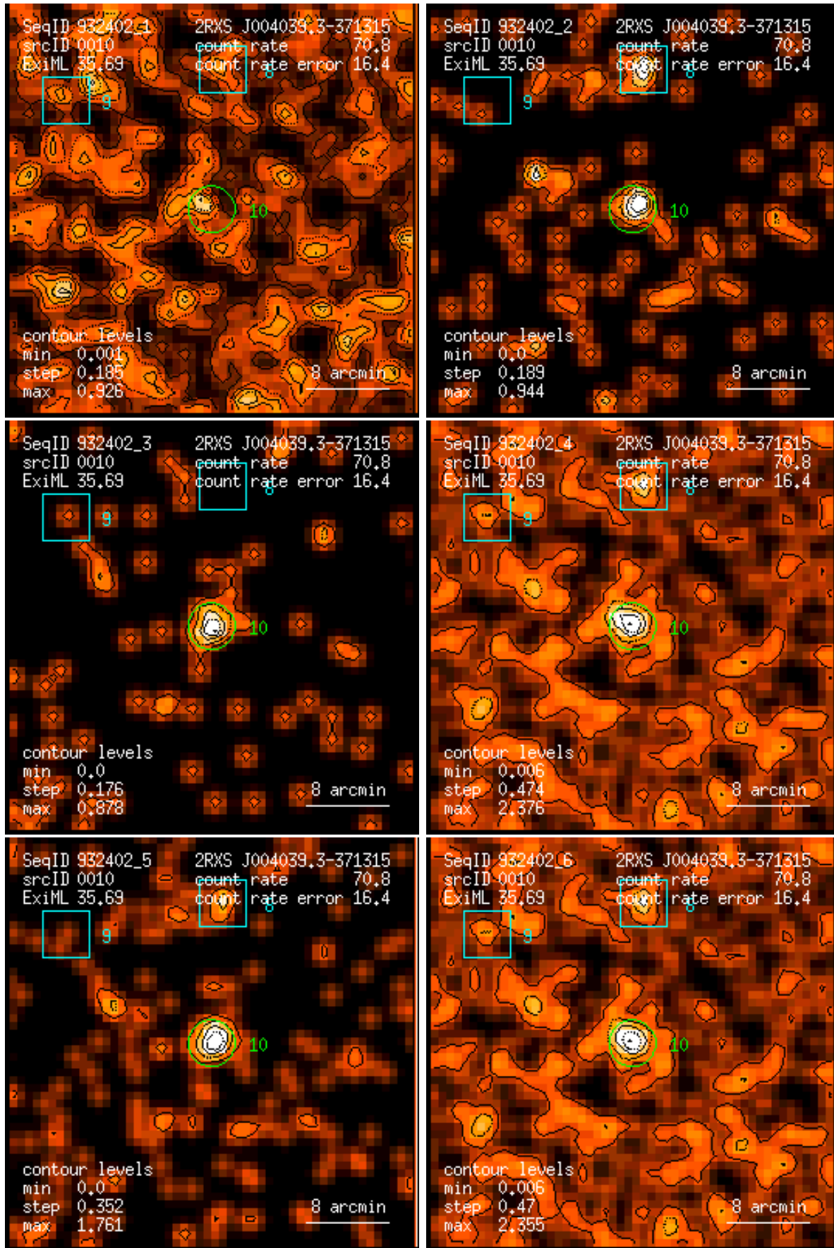
Figure 10: RASS 932402: detection 0010: band rate images, Gaussian filter: (1) PSPC channels 11 – 41, (2) 52 – 90, (3) 91 – 201, (4) 11 – 235, (5) 52 – 201, (6) 11 – 201. Broad band rates in counts/ks. Band rate contour levels in counts/ks/arcmin 2 .
