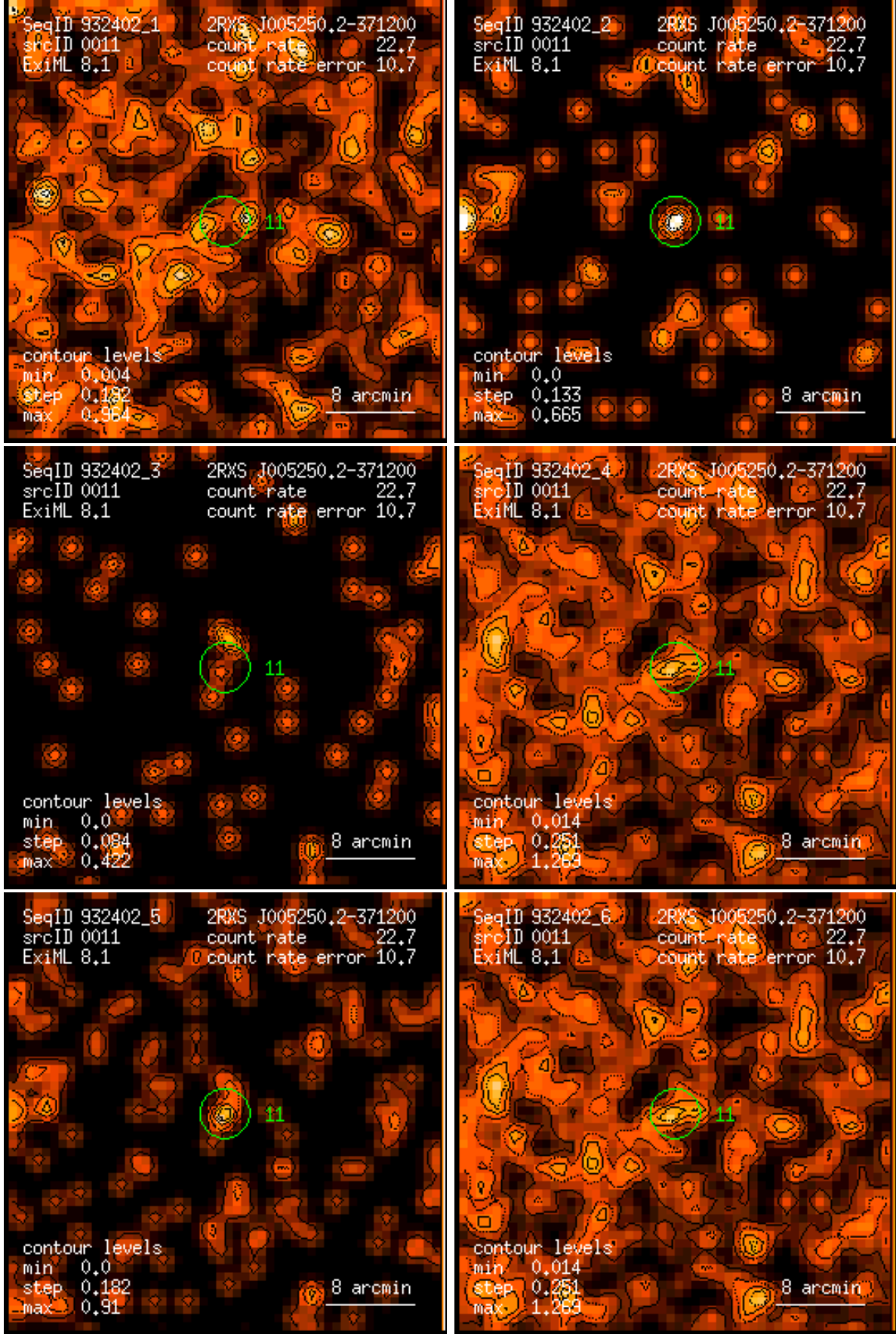
Figure 11: RASS 932402: detection 0011: band rate images, Gaussian filter: (1) PSPC channels 11 – 41, (2) 52 – 90, (3) 91 – 201, (4) 11 – 235, (5) 52 – 201, (6) 11 – 201. Broad band rates in counts/ks. Band rate contour levels in counts/ks/arcmin 2 .
