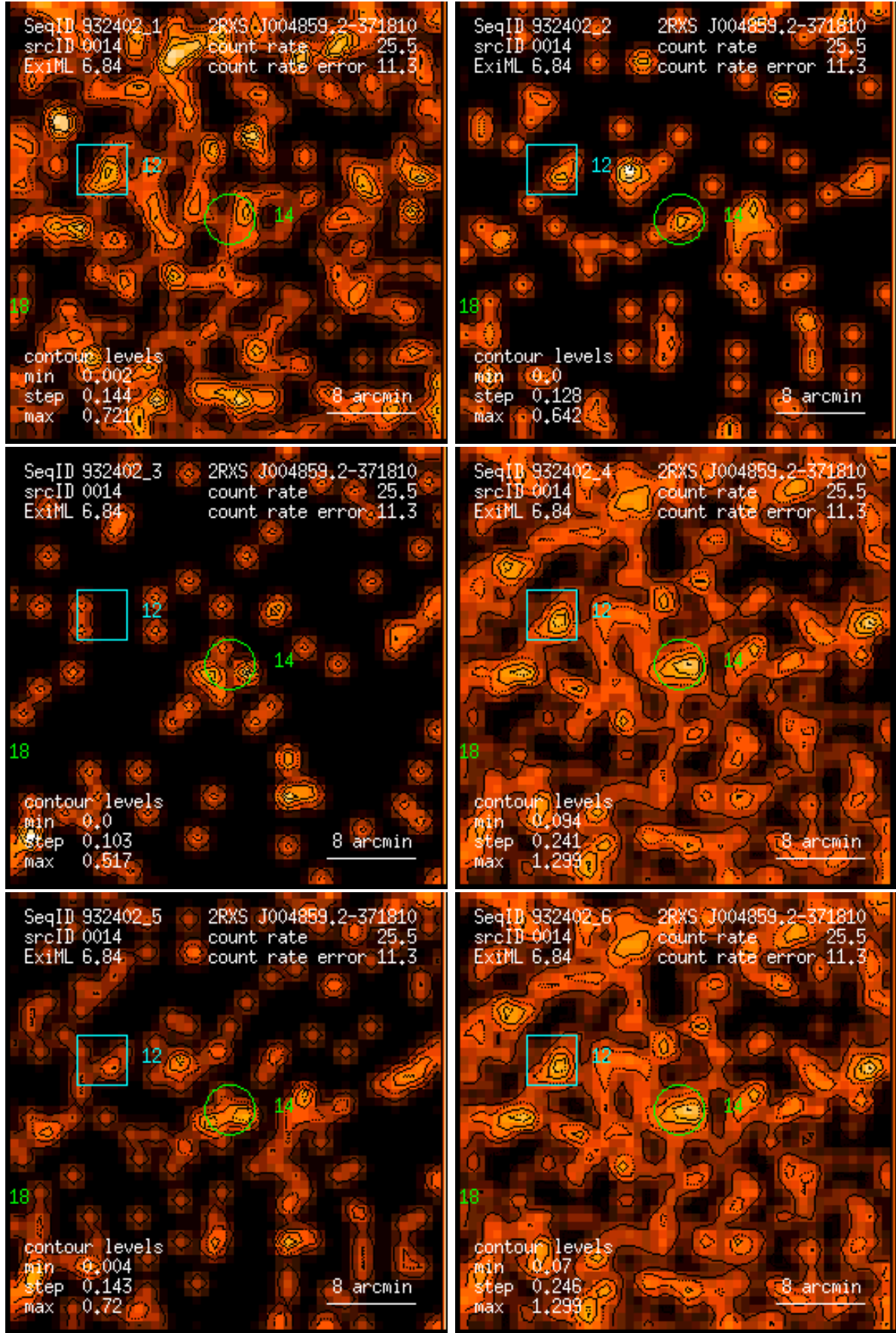
Figure 14: RASS 932402: detection 0014: band rate images, Gaussian filter: (1) PSPC channels 11 – 41, (2) 52 – 90, (3) 91 – 201, (4) 11 – 235, (5) 52 – 201, (6) 11 – 201. Broad band rates in counts/ks. Band rate contour levels in counts/ks/arcmin 2 .
