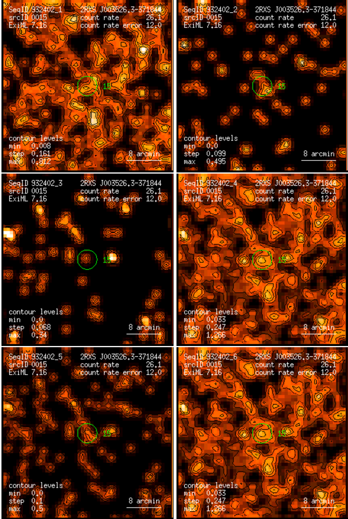
Figure 15: RASS 932402: detection 0015: band rate images, Gaussian filter: (1) PSPC channels 11 – 41, (2) 52 – 90, (3) 91 – 201, (4) 11 – 235, (5) 52 – 201, (6) 11 – 201. Broad band rates in counts/ks. Band rate contour levels in counts/ks/arcmin 2 .
