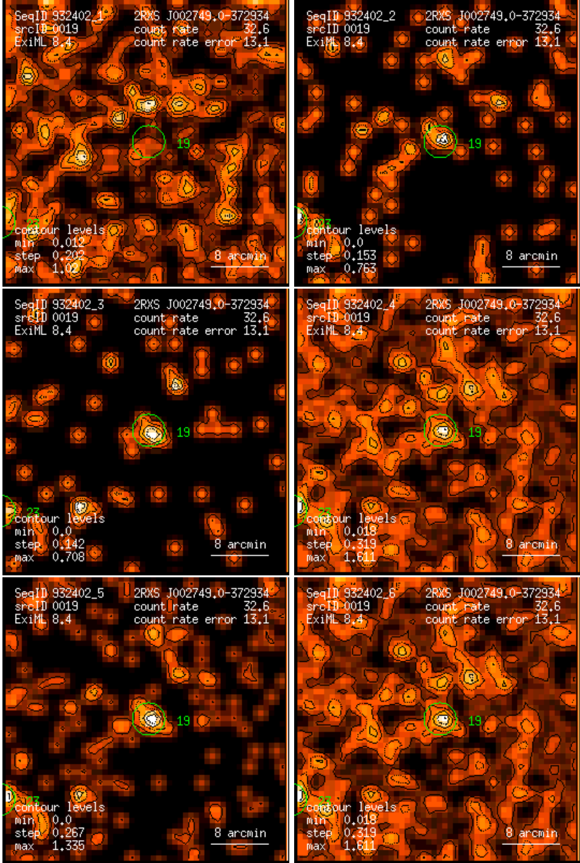
Figure 19: RASS 932402: detection 0019: band rate images, Gaussian filter: (1) PSPC channels 11 – 41, (2) 52 – 90, (3) 91 – 201, (4) 11 – 235, (5) 52 – 201, (6) 11 – 201. Broad band rates in counts/ks. Band rate contour levels in counts/ks/arcmin 2 .
