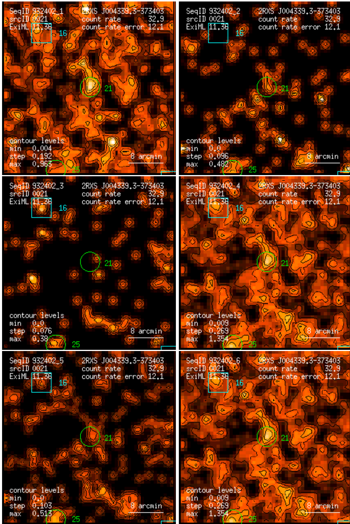
Figure 21: RASS 932402: detection 0021: band rate images, Gaussian filter: (1) PSPC channels 11 – 41, (2) 52 – 90, (3) 91 – 201, (4) 11 – 235, (5) 52 – 201, (6) 11 – 201. Broad band rates in counts/ks. Band rate contour levels in counts/ks/arcmin 2 .
