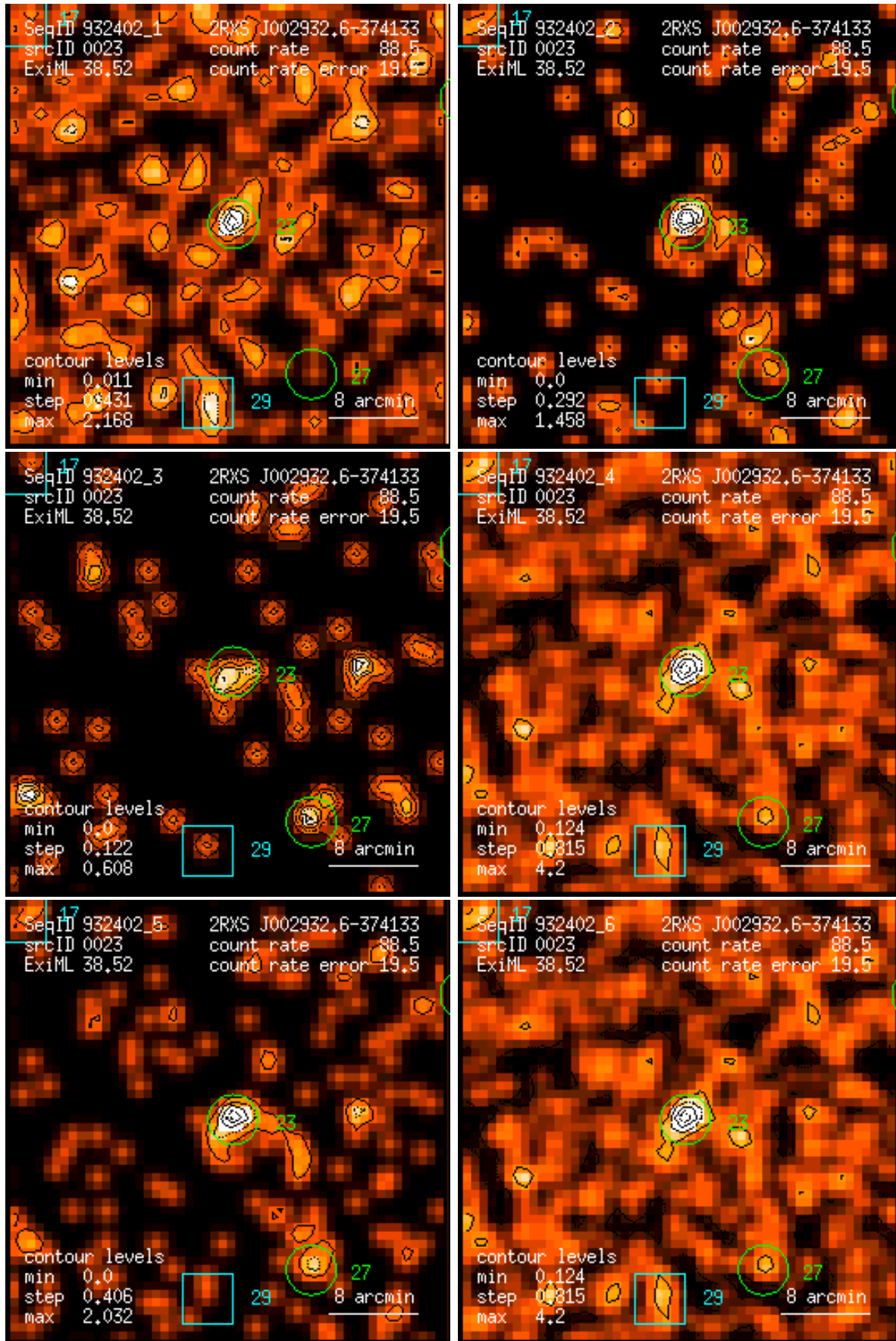
Figure 23: RASS 932402: detection 0023: band rate images, Gaussian filter: (1) PSPC channels 11 – 41, (2) 52 – 90, (3) 91 – 201, (4) 11 – 235, (5) 52 – 201, (6) 11 – 201. Broad band rates in counts/ks. Band rate contour levels in counts/ks/arcmin 2 .
