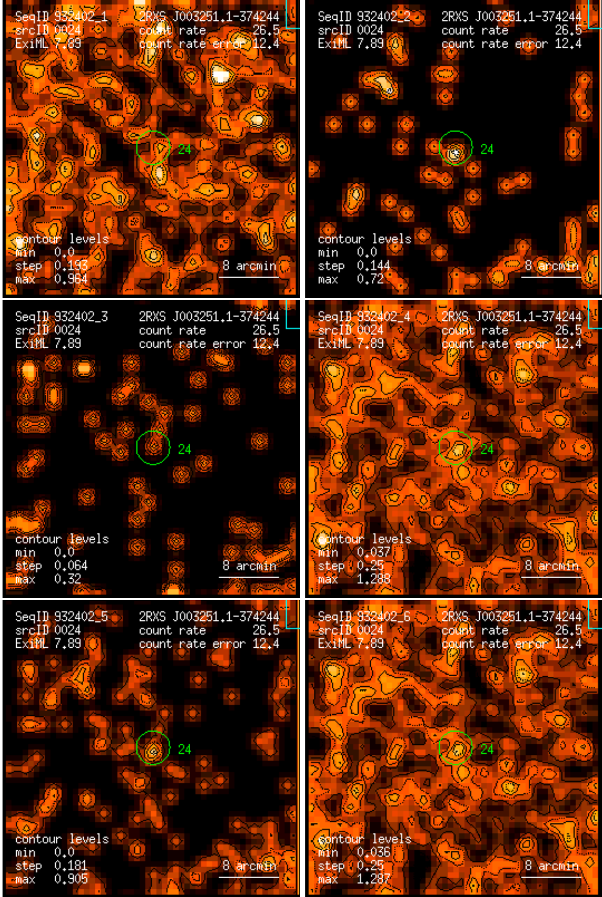
Figure 24: RASS 932402: detection 0024: band rate images, Gaussian filter: (1) PSPC channels 11 – 41, (2) 52 – 90, (3) 91 – 201, (4) 11 – 235, (5) 52 – 201, (6) 11 – 201. Broad band rates in counts/ks. Band rate contour levels in counts/ks/arcmin 2 .
