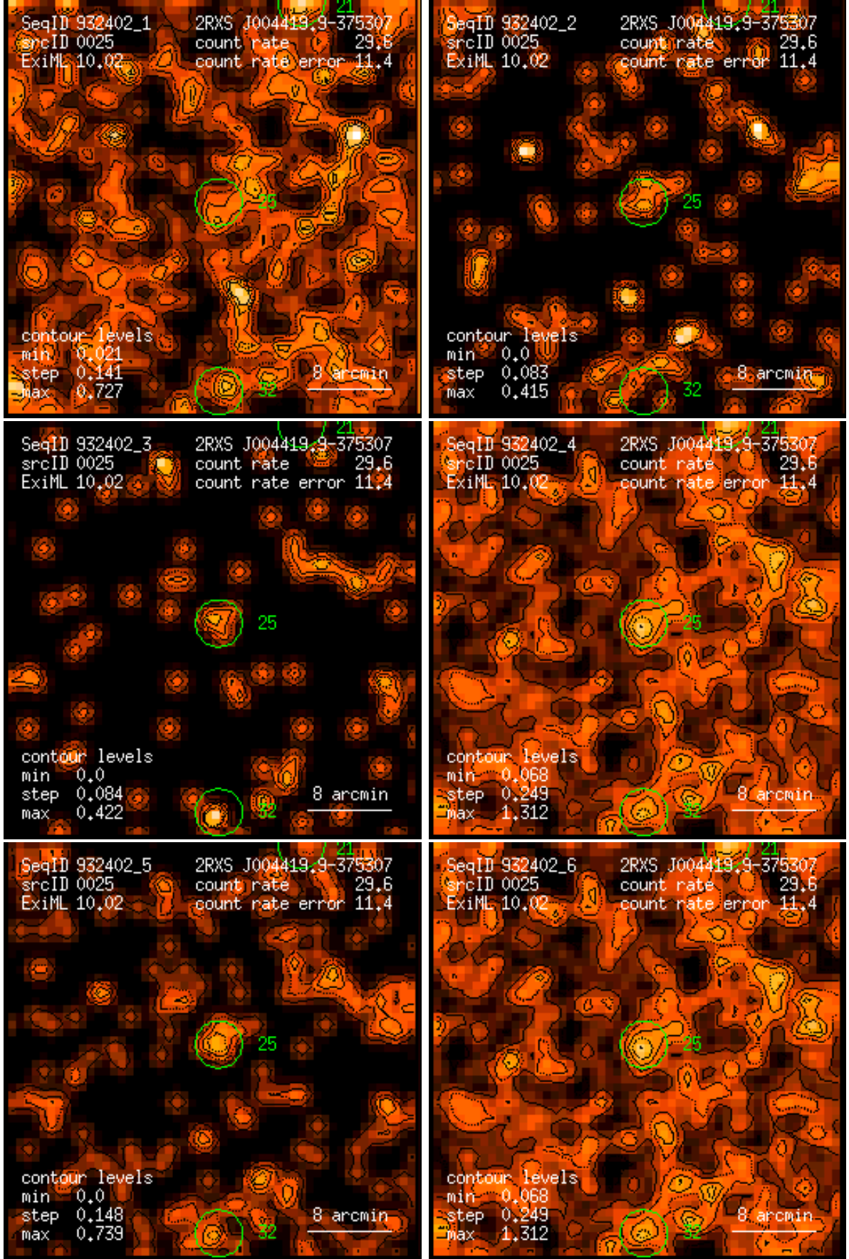
Figure 25: RASS 932402: detection 0025: band rate images, Gaussian filter: (1) PSPC channels 11 – 41, (2) 52 – 90, (3) 91 – 201, (4) 11 – 235, (5) 52 – 201, (6) 11 – 201. Broad band rates in counts/ks. Band rate contour levels in counts/ks/arcmin 2 .
