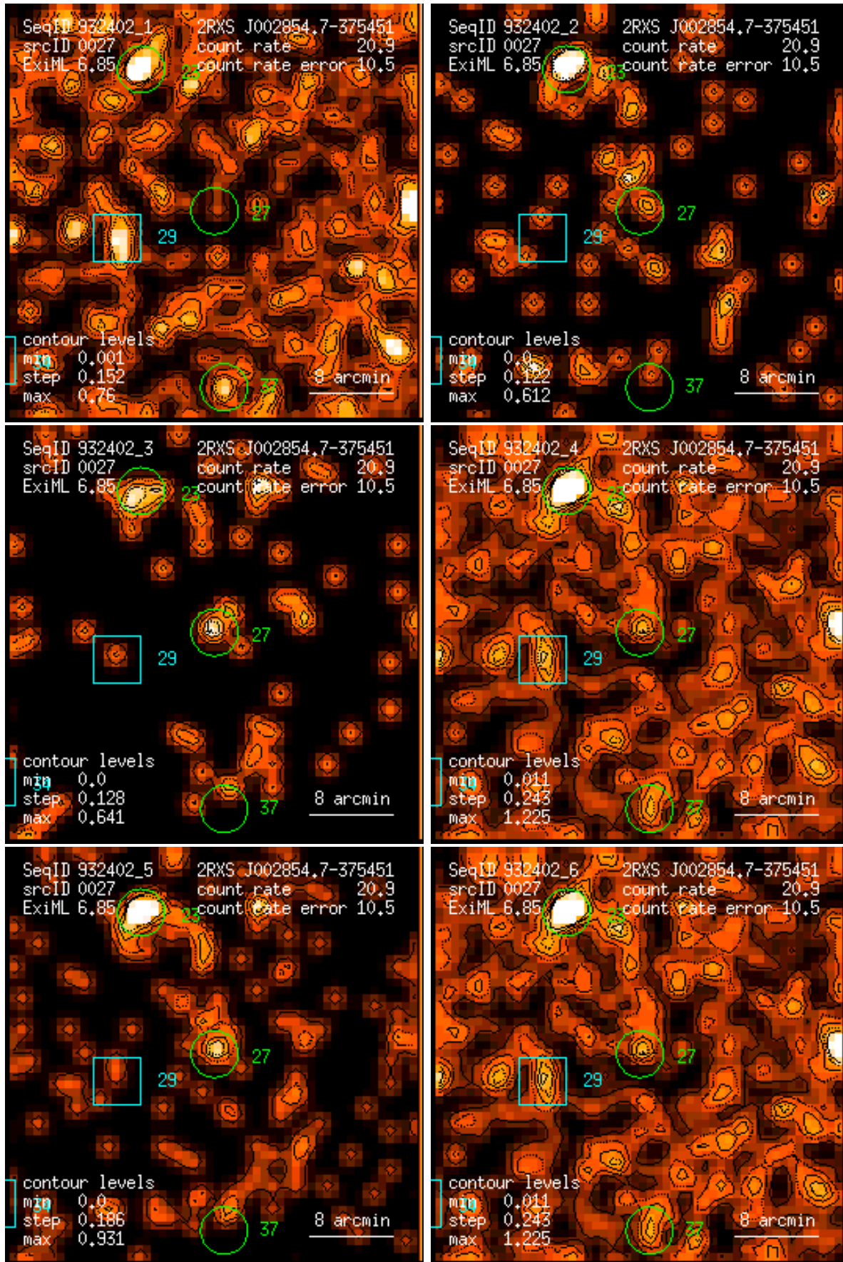
Figure 27: RASS 932402: detection 0027: band rate images, Gaussian filter: (1) PSPC channels 11 – 41, (2) 52 – 90, (3) 91 – 201, (4) 11 – 235, (5) 52 – 201, (6) 11 – 201. Broad band rates in counts/ks. Band rate contour levels in counts/ks/arcmin 2 .
