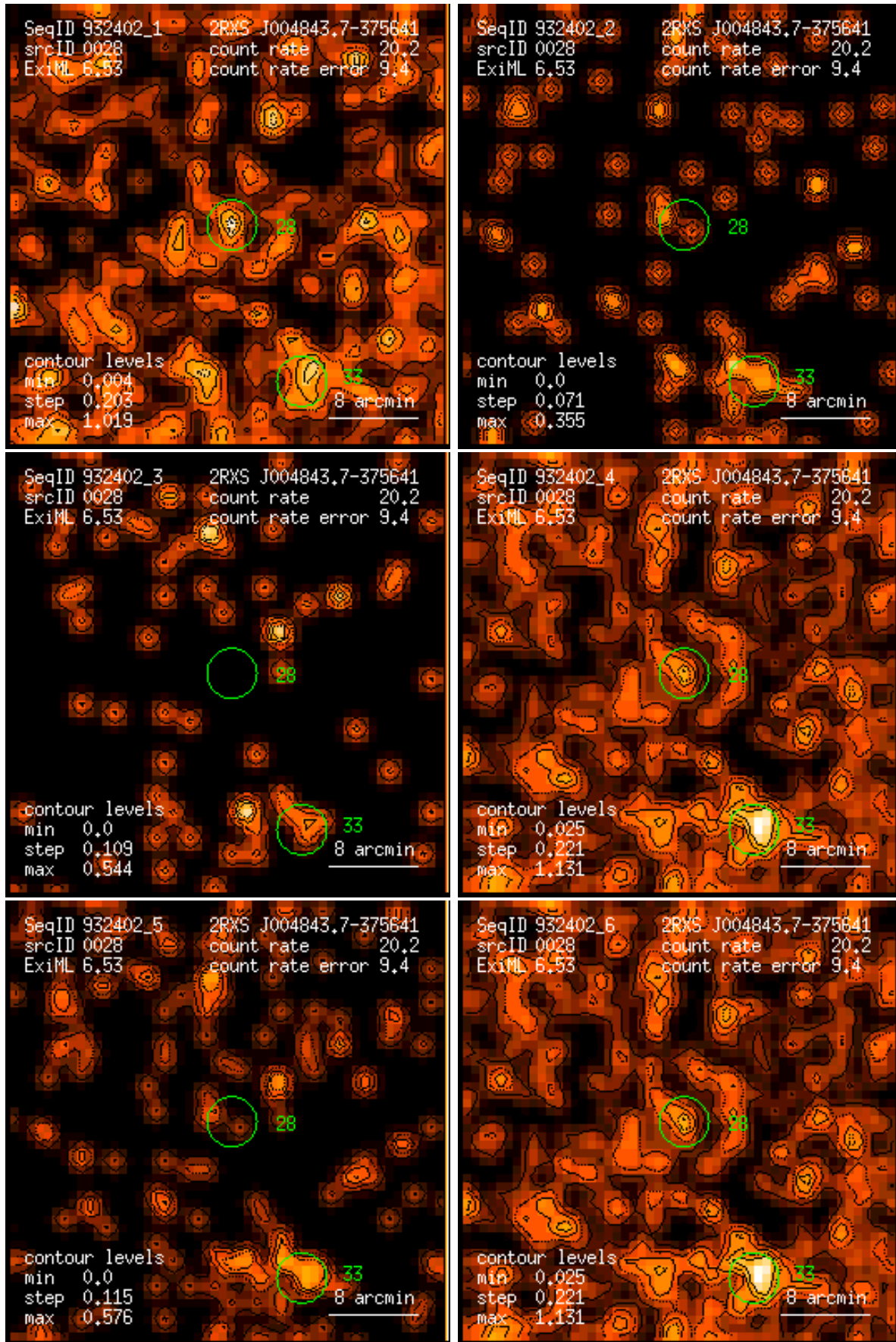
Figure 28: RASS 932402: detection 0028: band rate images, Gaussian filter: (1) PSPC channels 11 – 41, (2) 52 – 90, (3) 91 – 201, (4) 11 – 235, (5) 52 – 201, (6) 11 – 201. Broad band rates in counts/ks. Band rate contour levels in counts/ks/arcmin 2 .
