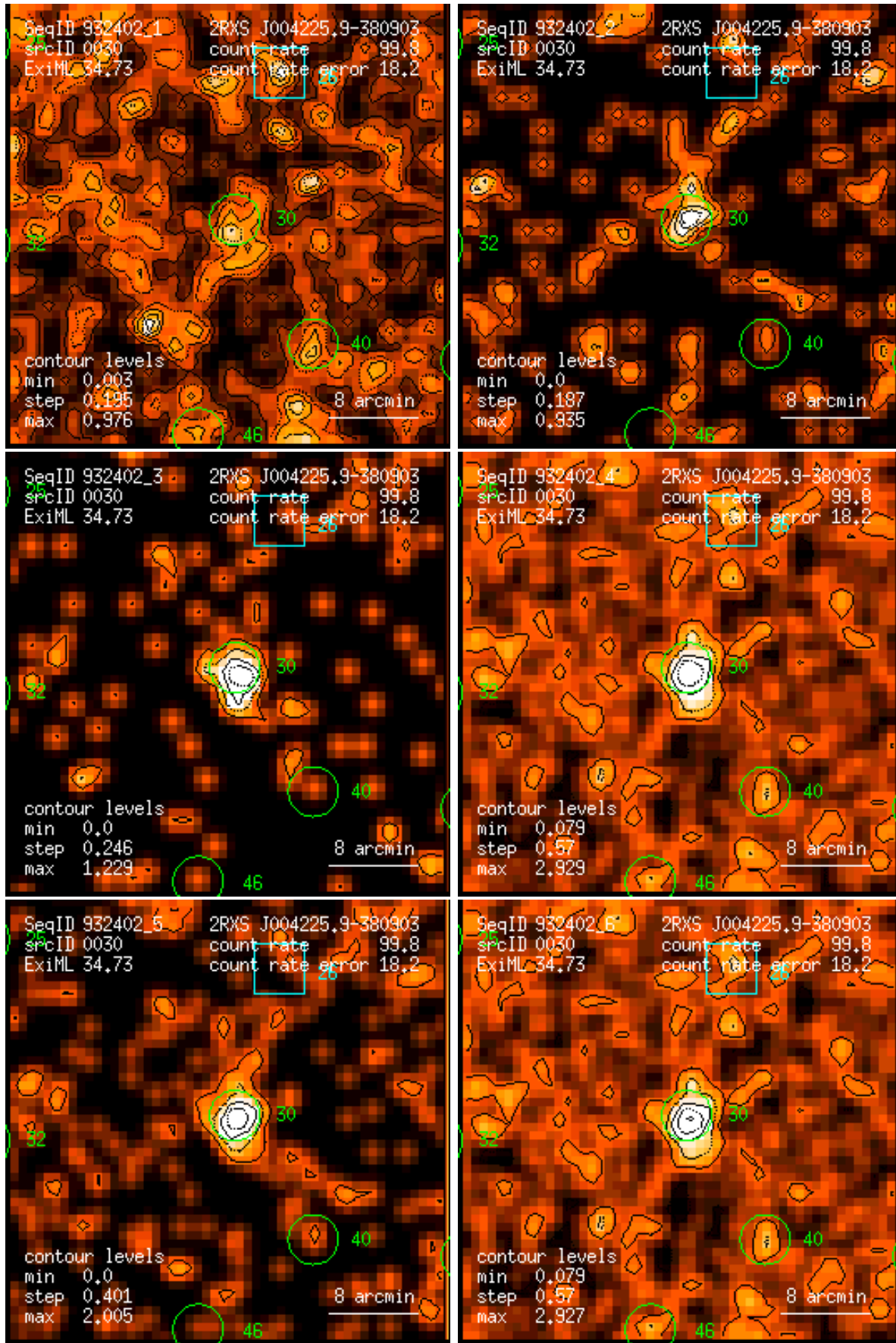
Figure 30: RASS 932402: detection 0030: band rate images, Gaussian filter: (1) PSPC channels 11 – 41, (2) 52 – 90, (3) 91 – 201, (4) 11 – 235, (5) 52 – 201, (6) 11 – 201. Broad band rates in counts/ks. Band rate contour levels in counts/ks/arcmin 2 .
