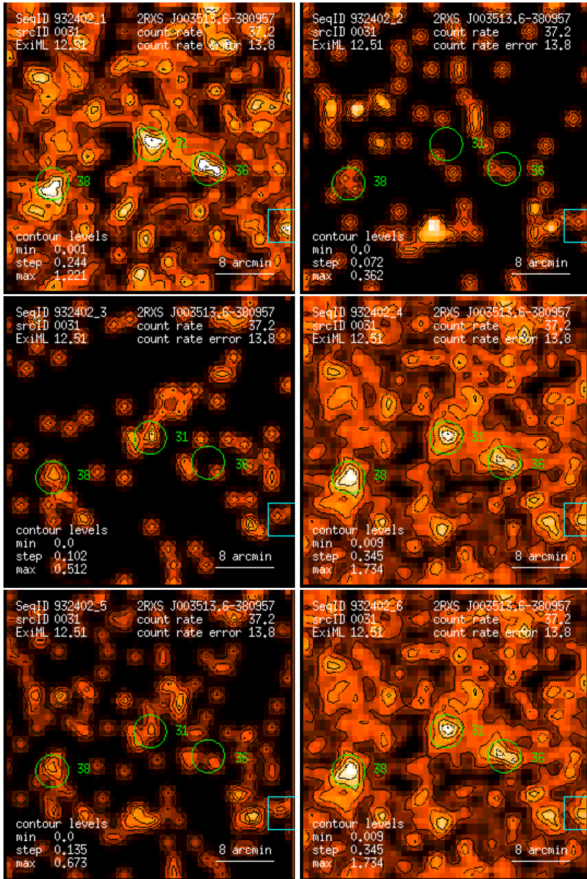
Figure 31: RASS 932402: detection 0031: band rate images, Gaussian filter: (1) PSPC channels 11 – 41, (2) 52 – 90, (3) 91 – 201, (4) 11 – 235, (5) 52 – 201, (6) 11 – 201. Broad band rates in counts/ks. Band rate contour levels in counts/ks/arcmin 2 .
