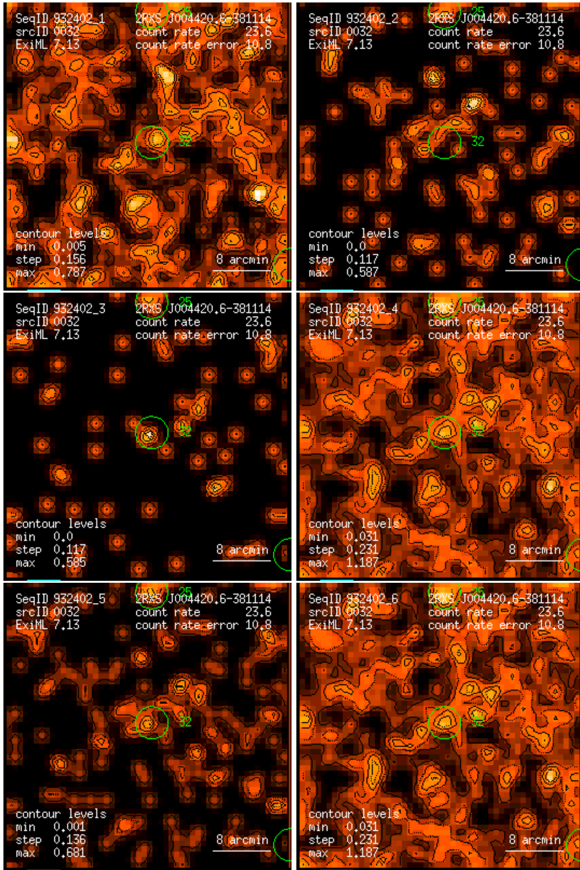
Figure 32: RASS 932402: detection 0032: band rate images, Gaussian filter: (1) PSPC channels 11 – 41, (2) 52 – 90, (3) 91 – 201, (4) 11 – 235, (5) 52 – 201, (6) 11 – 201. Broad band rates in counts/ks. Band rate contour levels in counts/ks/arcmin 2 .
