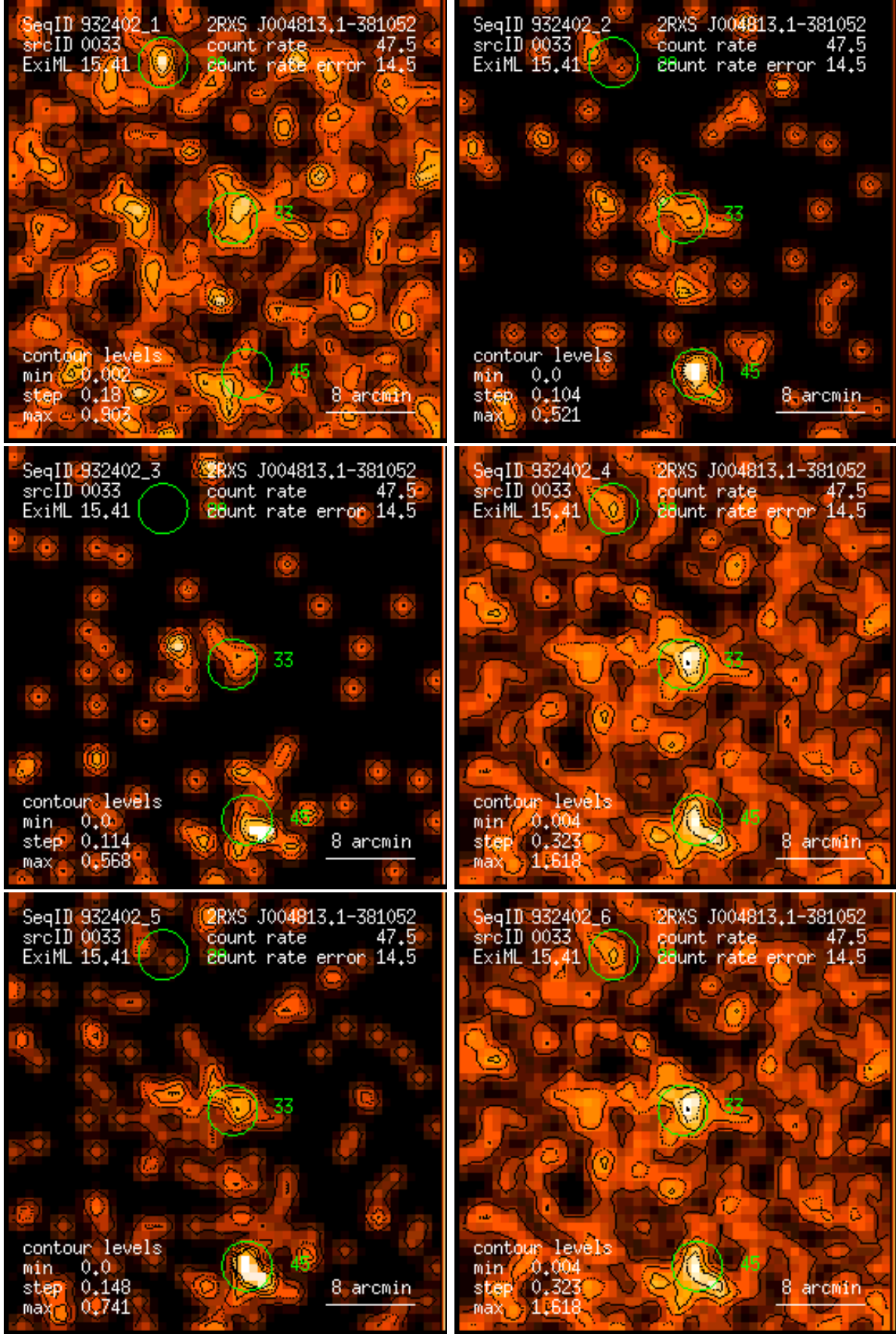
Figure 33: RASS 932402: detection 0033: band rate images, Gaussian filter: (1) PSPC channels 11 – 41, (2) 52 – 90, (3) 91 – 201, (4) 11 – 235, (5) 52 – 201, (6) 11 – 201. Broad band rates in counts/ks. Band rate contour levels in counts/ks/arcmin 2 .
